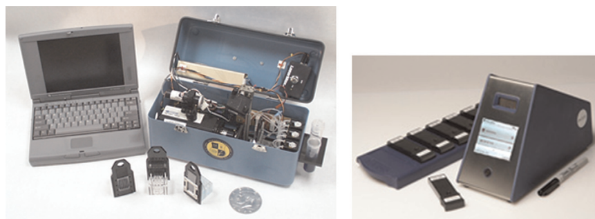
Fig. 3. Planar waveguide biosensors for fluorescence detection in the evanescent region: NRL system (left) and mBio (right).
