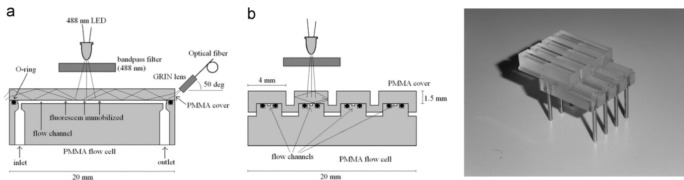
Fig. 2. Integrating waveguide capillary sensor (Baldini et al., 2008). Schematics a and b diagram the waveguide and channel from the side and end, respectively, while a photo of a 4-channel device is shown on the right. Reprinted with permission from IEEE.
