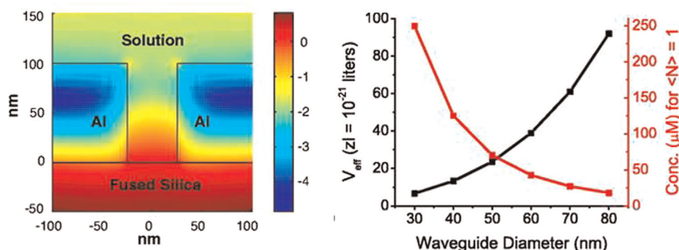
Fig. 5. Zero mode waveguides (Levene et al., 2003). Left: Simulation of the log of the intensity distribution for a zero-mode waveguide 50 nm in diameter and 100 nm long. Right: The effective volume V_{\text{eff}} and the corresponding concentration for which an average of one molecule enters the volume. Reprinted with permission from Science.
