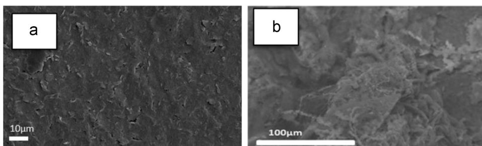
Fig. 1. (a) SEM image of the working electrode from a SPBGE platform; (b) SEM image of the film formed by MWCNTs/FcMe/CS/HRP/BSA/LOx composite film on the working electrode surface of the SPBGE electrochemical platform.
