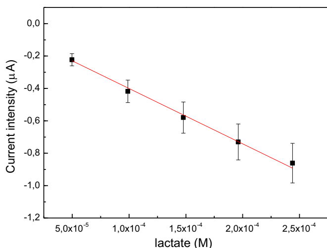
Fig. 5. Reproducibility study for the lactate calibration plot ( R=0.99781 , n=8 electrochemical lactate biosensors) in 0.1 M PBS pH 7.4 at 22\text{ }^{\circ}\text{C} and -0.2\text{ V} .
