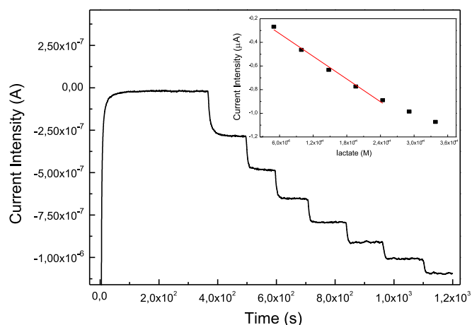
Fig. 4. Chronoamperometric response of the electrochemical lactate biosensor with a successive addition of 25 \mu\text{L} of a 10 mM lactate solution in 0.1 M PBS solution pH 7.4 at working potential of -0.2\text{ V} . Inset of figure: calibration plot of the response electrochemical lactate biosensor with lactate concentration in 0.1 M PBS pH 7.4 at -0.2\text{ V} and 22\text{ }^{\circ}\text{C} .
