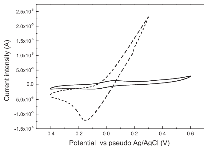
Fig. 2. Cyclic voltammograms of the electrochemical lactate biosensor in the absence of CS (solid line) and in the presence of CS (dashed line) in 0.1 M PBS pH 7.4 at 22^\circ\text{C} . Scan rate 10 \text{ mV s}^{-1} . First scan recorded.
