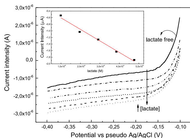
Fig. 3. Linear sweep voltammetry response for the electrochemical lactate biosensor with a successive addition of 50 \mu\text{L} of a 10 \text{ mM} lactate solution in 0.1 \text{ M} PBS solution pH 7.4 under hydrodynamic conditions. Scan rate was 10 \text{ mV s}^{-1} . Inset of figure: calibration plot for the electrochemical lactate biosensor with lactate concentration in 0.1 \text{ M} PBS pH 7.4 at a working potential of -0.2 \text{ V} and 22^\circ\text{C} .
