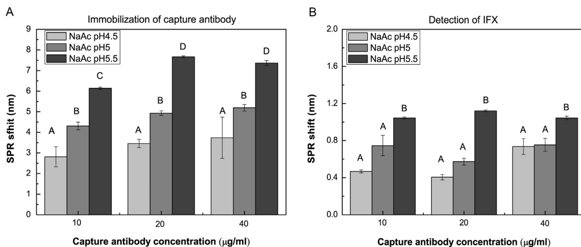
Fig. 2. Results of immobilization. Summary of immobilization shifts for 10, 20 and 40 \mu\text{g/ml} of the capture antibody diluted in buffer with three different pH values (A), and corresponding SPR shifts for detection of 10 \mu\text{g/ml} of IFX (B). Error bars represent standard deviation ( n=3 ). Threshold letters (A, B, C and D) indicate statistically significant differences from Bonferroni correction.
