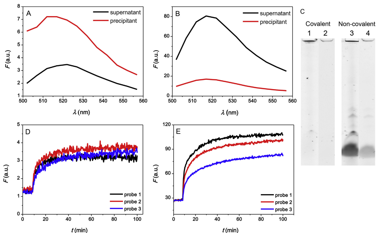
Fig. 3. Fluorescence spectra of (A) the covalent and (B) the non-covalent probe 3 sensors after reaction with 1 \mu\text{M} \text{Hg}^{2+} and centrifugation. The precipitants were re-dispersed in the same buffer. (C) Gel images of the covalent (lane 1, 2) and noncovalent (lane 3, 4) probe 3 sensors after reaction with 1 \mu\text{M} \text{Hg}^{2+} before (lane 1, 3) and after centrifugation (lane 2, 4). Kinetics of fluorescence increase for (D) the covalent and (E) the non-covalent sensors in the presence of 1 \mu\text{M} \text{Hg}^{2+} added at 10 min. Buffer: 150 mM \text{NaNO}_3 , 25 mM HEPES, pH 8.0.
