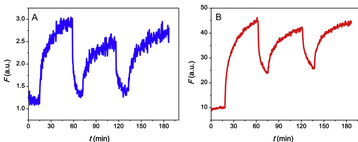
Fig. 6. Relative fluorescence signaling of (A) the covalent sensor and (B) the non-covalent sensor for continuous monitoring of \text{Hg}^{2+} concentration after adding 1\ \mu\text{M}\ \text{Hg}^{2+} at 15 min, 5\ \mu\text{M}\ \text{I}^- at 60 min, 10\ \mu\text{M}\ \text{Hg}^{2+} at 73 min, 5\ \mu\text{M}\ \text{I}^- at 117 min and 10\ \mu\text{M}\ \text{Hg}^{2+} at 133 min. Buffer: 150 mM \text{NaNO}_3 , 25 mM HEPES, pH 8.
