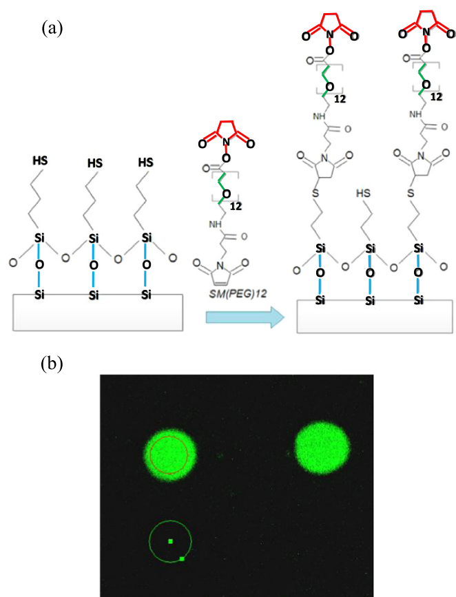
Fig. 2. (a) Schematic representation of the surface chemistry for NHS activation on the SiN surface. Blue (Si–O–Si): siloxane functional group; red (C 4 H 5 NO 3 ): NHS ester; green ((O–CH 2 –CH 2 ) 12 ): PEG. (b) A fluorescence microscope image showing selective binding of CTB to GM1 glycan with negligible binding to the areas lacking GM1 (but having a PEG brush). The average fluorescence signal intensity is about two orders of magnitude larger in the areas containing GM1 receptors than otherwise. (For interpretation of the references to color in this figure caption, the reader is referred to the web version of this paper.)
