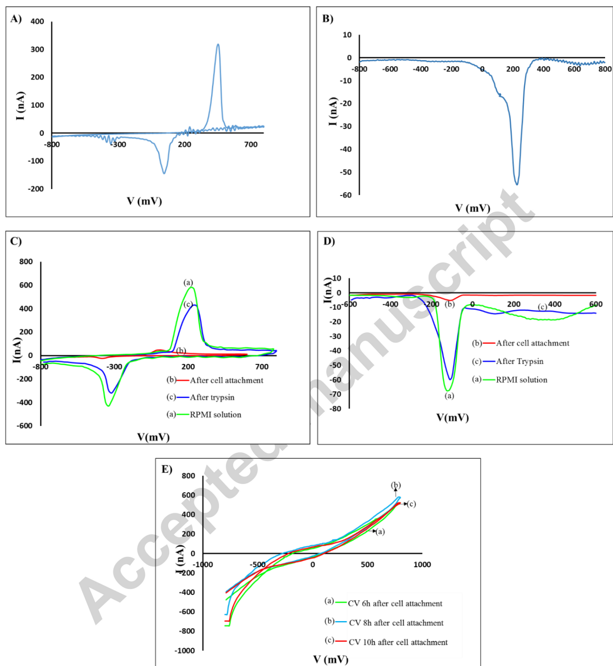
Figure 2. A) CV and B) DPV of ferricyanide ( K_3Fe(CN)_6 ) as standard ionic solution measured by SiNW electrochemical biosensor. C) CV and D) DPV of SiNW biosensor before and after attachment of MCF-7 cells as well as after their detachment from the surface by trypsin. .E) CV response of cells attached on SiNWEs in various time laps. It presented the stable electrochemical state for the cells after attachment on the sensor.
