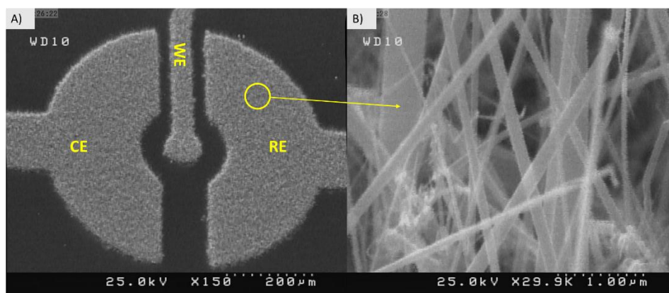
Figure 1. A,B) FESEM image of SiNW biosensor. The NWs just existed in the patterned region.
