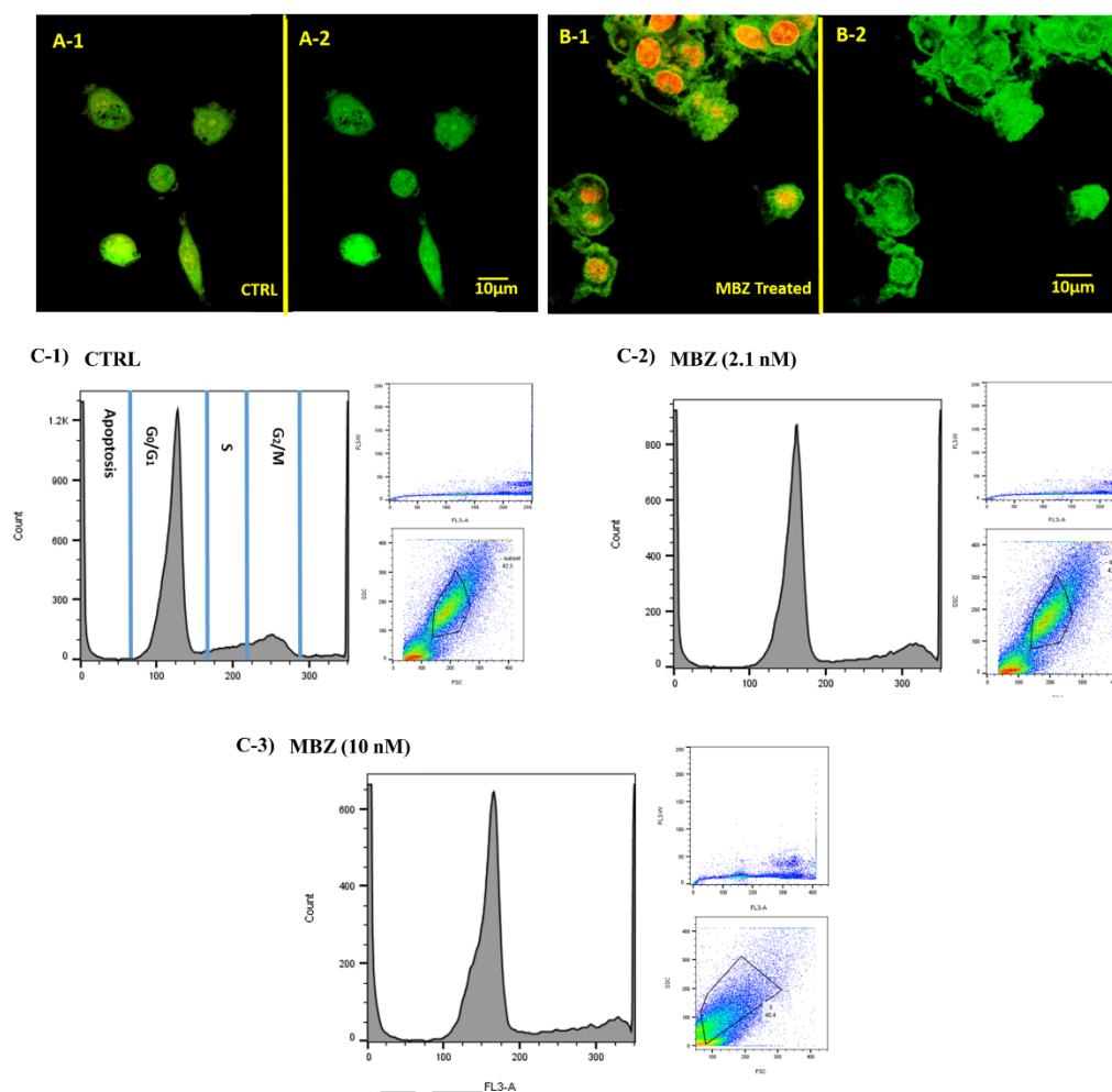
Figure 6 -Confocal microscopy images from the tubulin assemblies of MCF-7 cells in (A) CTRL state in comparison with (B) the cells treated by 2.1 nM of MBZ in same times. The duration of incubation with drugs was 2h. Extensive depolymerization rate in MTs resulted in non-regular spindle formation in MBZ treated samples the trace of the PI tagged nucleus is observable in panels A-1 and B-1 in orange color. Also, flowcytometry analyses of MCF-7 cells in (C-1) No drug, (C-2) MBZ 2.1 nM and (C-3) MBZ 10,5 nM treated states were presented. The cell's fractions in apoptotic, G 0 /G 1 , S and G 2 /M cycles are observable in all of panels. MBZ treatment reduced the vitality of the cells and perturb the cells cycle. R1 region (presented in the right of each panels) indicated the state of counted cells.
