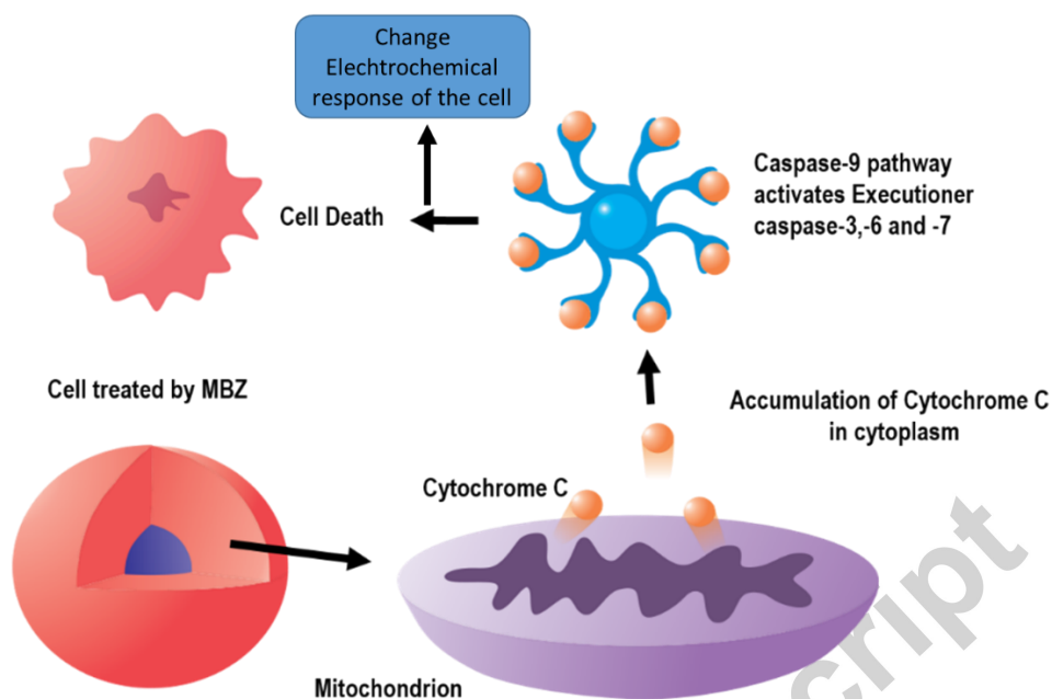
Figure 5- Schematics from the electrochemical effect of MBZ on MCF-7 cells. Accumulation of cytochrome C from the mitochondria to the cytoplasm resulted in perturbation of the cell's ionic or electrochemical state.
