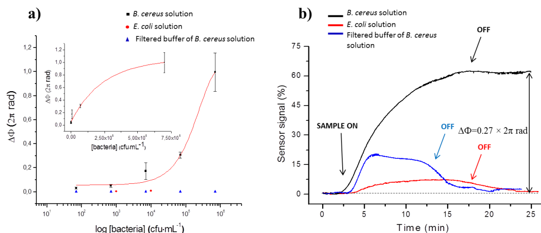
Fig. 2 (a) Calibration curve for the detection of triplicate logarithmic concentrations of B. cereus bacteria (black, squares) ranging from 70 to 7 \times 10^5 \text{ cfu}\cdot\text{mL}^{-1} [the exponential fit equation is given by y = 1.05 - 0.99 \cdot e^{(-4.13 \times 10^{-6} x)} ] in comparison with non-specific bacteria E. Coli (red, circles) at concentrations of 1 \times 10^3 \text{ cfu}\cdot\text{mL}^{-1} and 1 \times 10^4 \text{ cfu}\cdot\text{mL}^{-1} and concentrations of filtered buffer from B. Cereus solutions (blue, triangles) ranging from 70 to 7 \times 10^5 \text{ cfu}\cdot\text{mL}^{-1} . In the inset: linear representation of the data for the B. Cereus detection [linear regression of the linear part is given by y = 2.18 \cdot 10^{-5} x + 0.031 , r^2 = 0.94521 ] and (b) real-time detection of specific B. cereus solution at a concentration of 7 \times 10^3 \text{ cfu}\cdot\text{mL}^{-1} (black line), non-specific E. coli solution at a concentration of 1 \times 10^4 \text{ cfu}\cdot\text{mL}^{-1} (red line) and filtered buffer from B. cereus solution at a concentration of 7 \times 10^3 \text{ cfu}\cdot\text{mL}^{-1} (blue line) by a direct immunoassay in PBST buffer.
