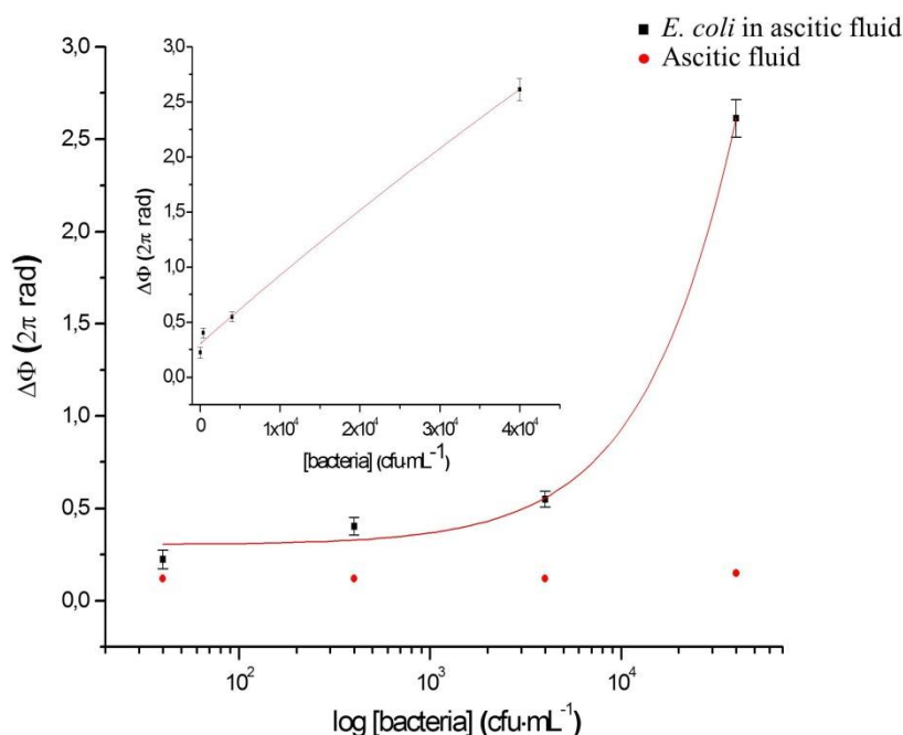
Fig. 5 Calibration curve for triplicate spiked concentrations of E. coli ranging from 40 and 4 \times 10^4 \text{cfu}\cdot\text{mL}^{-1} in ascitic fluid (black, squares) [the exponential fit equation is given by y = 12.5 - 12.2 \cdot e^{(-5.3 \times 10^{-6} x)} ] and unspecific detection of pure ascitic fluid. In the inset: linear representation of the data for E. Coli detection [the linear regression is given by y = 5.7 \cdot 10^{-5} x + 0.3 , r^2 = 0.982 ].
