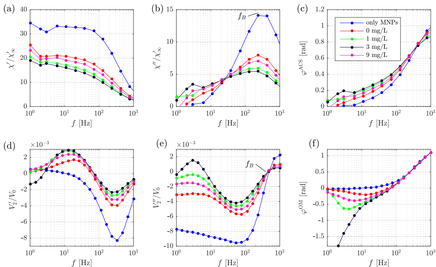
Fig. 2. Results of agglutination assay measurements for anti-CRP functionalized beads in blocking buffer (blue), and in a mixture of 190 \mu L MNP suspension with 20 \mu L CRP-free serum with CRP concentrations c of < 0.02 mg/L (red), 1 mg/L (green), 3 mg/L (black) and 9 mg/L (pink). Panels (a) and (b) show the real and imaginary components \chi' and \chi'' of the magnetic susceptibility normalized with the high-frequency value of the in-phase susceptibility \chi_\infty and panel (c) shows the corresponding magnetic phase lag \phi^{\text{ACS}} = \text{atan2}(\chi'', \chi') . Panels (d) and (e) show the real and imaginary components V_2' and V_2'' of the optomagnetic signal normalized with the total light intensity V_0 and panel (f) shows the corresponding magnetic phase lag, \phi^{\text{OM}} = \text{atan2}(-V_2', -V_2'')/2 . Data in (a)–(c) represent single measurements. Data in (d)–(f) represent three consecutive measurements on the same sample with error bars smaller than the shown data points. The lines are guides to the eye.
