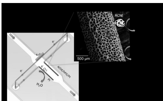
Figure 1. Design and working principle of the AChE fuel cell. The fuel cell consists of a membrane-less single channel that operates in flow-through mode. The cell hosts an anode (Pt wire coated with a film of highly porous gold, hPG) and a cathode, (Pt wire) connected to a external circuit with a fixed external load ( R_{ext} ). AChE is immobilised onto the anode surface and catalyses the first step of oxidation of ACh, while hPG catalyses the
