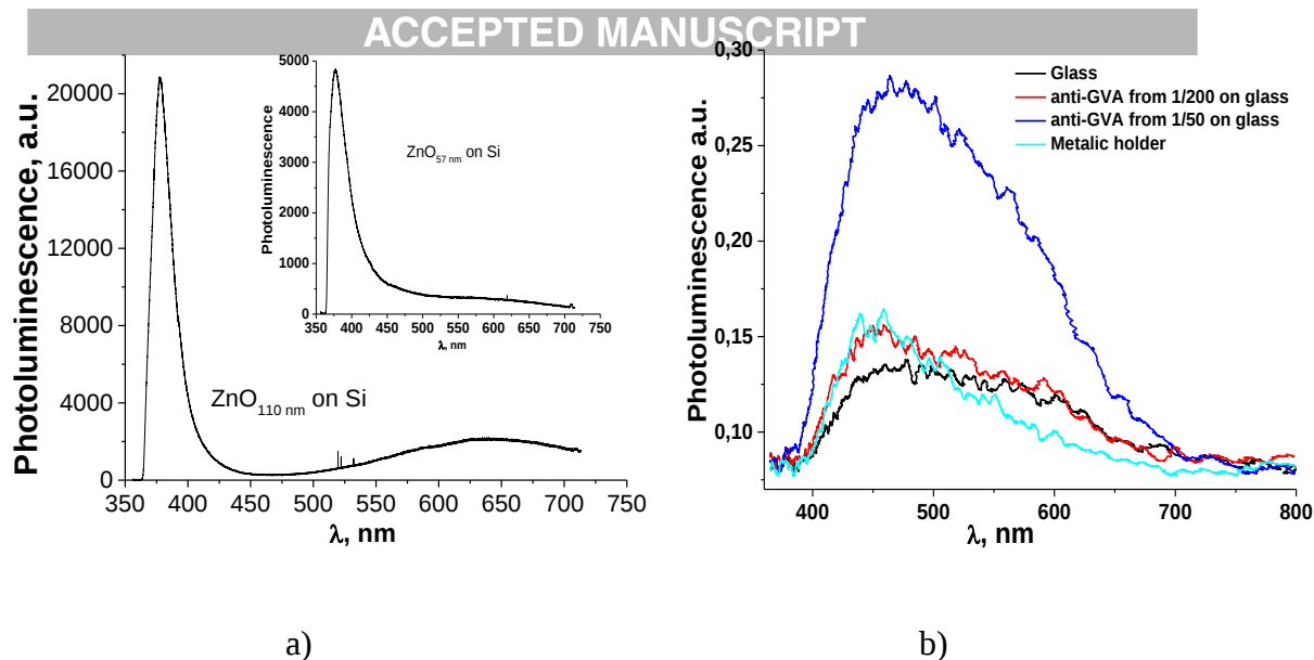
Figure 2. PL spectra of the ZnO samples with 57 and 110 nm layer thicknesses (a), PL spectra of anti-GVA deposited on glass (b).
