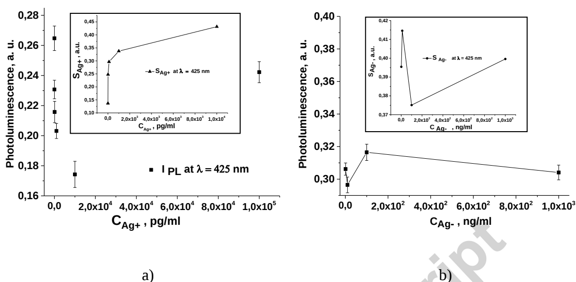
Figure 6. PL intensity at 425 nm as a function of GVA-antigen concentration in Ag+ specimen, inset – biosensor response (S) as a function of GVA-antigen concentration in Ag+ specimen (a), PL intensity at 425 nm as a function of different concentrations of proteins separated from healthy vine grapes, which not contain any antigen capable to bind with anti-GVA (specimens – Ag-), inset - biosensor response (S) as a function of Ag- specimen concentration (b).
