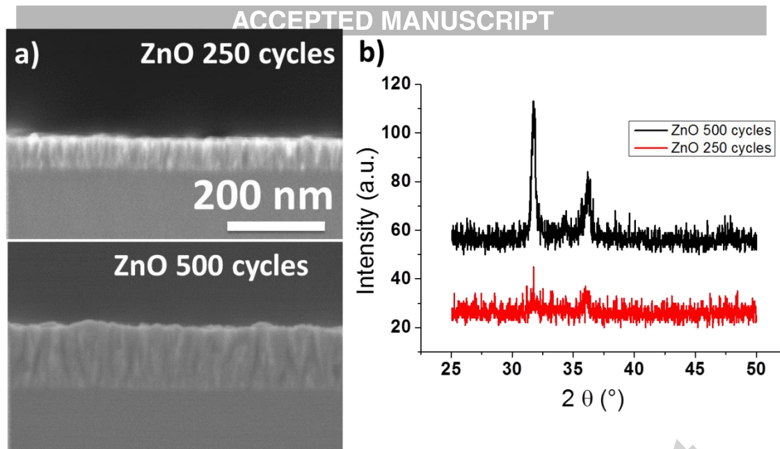
Figure 1. a) SEM cross section images and b) GIXRD of ZnO ALD films deposited on Si substrates by different numbers of cycles (250 and 500).
