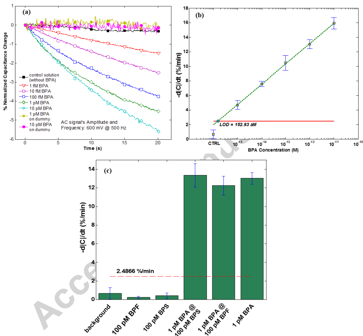
Figure 4. (a) Normalized C_{int} changes with time for blank buffer, dummy electrodes and different concentrations of BPA. (b) Sensor response to different concentrations of BPA samples. The dotted line is the extracted standard curve. Its slope represents the sensor sensitivity. The horizontal line indicates the LOD ( 152.93 aM) of the sensor. Error bars represent standard deviation. (c) Sensor specificity. The response of the sensor for the background, 100 pM BPF and 100 pM BPS are below the cut-off line. The sensor response for 1 pM BPA in the presence of 100 pM BPs and BPF is very close to the sensor response to 1 pM BPA. High resolution version of the figures are provided in Figures S6 to S8 of the Supplementary Materials.
