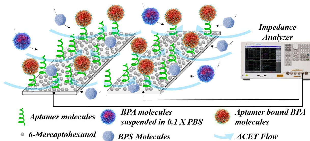
Figure 3. Excitation of ACET effect is integrated into capacitance measurement during a BPA detection experiment. The ACET flows carry BPA particles toward functionalized sites and accelerate the sensor response.
