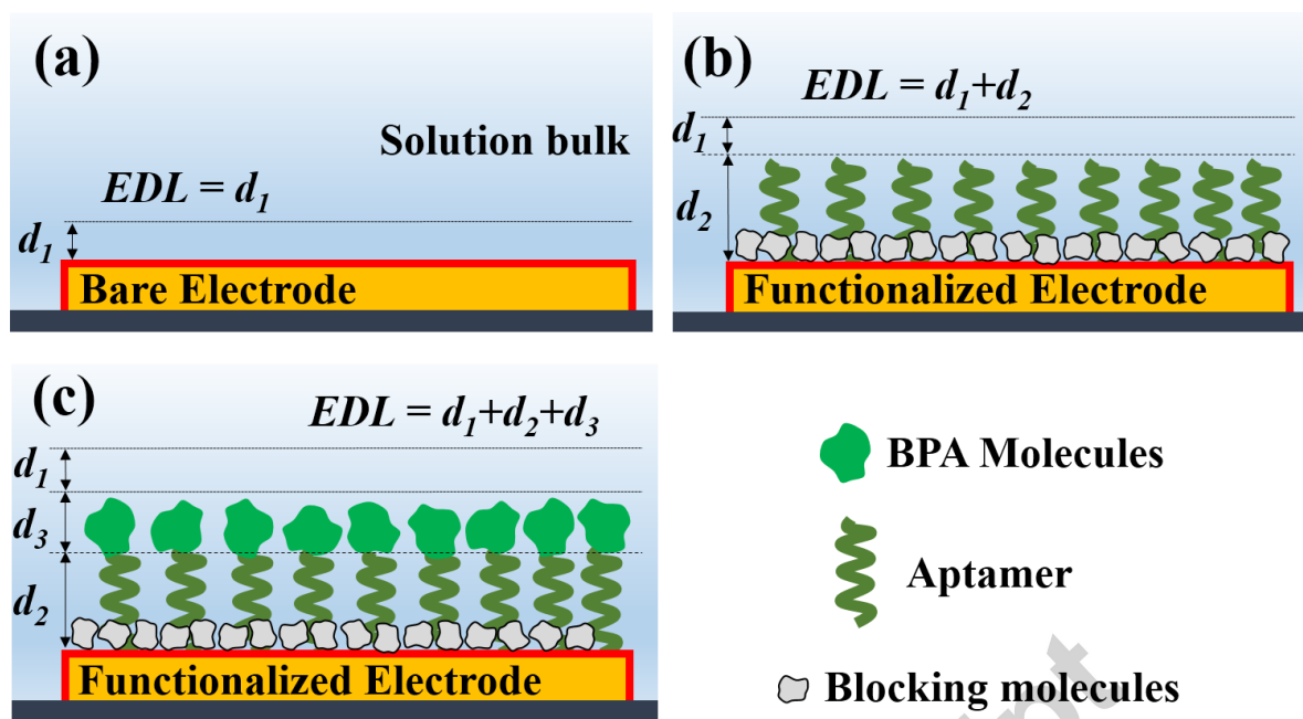
Figure 1. Changes in EDL layer of the electrodes at different stages of sensor functionalization and BPA binding. (a) The electrode is clean but not functionalized, and the EDL thickness is d_1 . (b) The electrode is functionalized, and the EDL thickness becomes d_1 + d_2 . (c) After binding reaction happens and BPA molecules bind to the aptamer, EDL thickness increase to d_1 + d_2 + d_3 .
