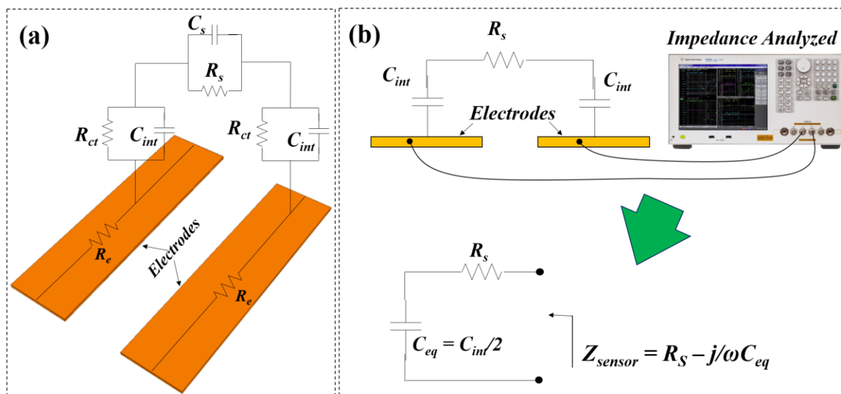
Figure 2. (a) Equivalent circuit model of two nearby electrodes in an IDE sensor. (b) Simplified equivalent circuit model of the sensor at frequencies lower than 100 kHz.
