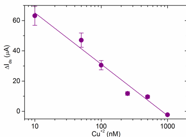
Fig. 5 \Delta I_{ds} as a function of the \text{Cu}^{+2} concentration for a (PEI/Urease) 3 LbL assembly. The \text{Cu}^{+2} solutions contained 0.2 mM urea. Experimental conditions: 10 mM KCl and 0.1 mM HEPES at pH 6, flow rate = 300 \mu\text{l}/\text{min} , V_g = -0.2 V and V_{ds} = 0.1 V. Error bars represent the standard deviation from measurements performed using three different devices.
