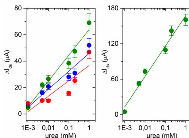
Fig. 4 (a) \Delta I_{ds} of the flow response (flow rate = 300 \mu l/min ) as a function of the urea concentration for (PEI/Urease) 1 (red), (PEI/Urease) 2 (blue) and (PEI/Urease) 3 (green) LbL assemblies. (b) \Delta I_{ds} of the static response as a function of the urea concentration for a (PEI/Urease) 3 LbL assembly. Experimental conditions: 10 mM KCl and 0.1 mM HEPES at pH 6, V_g = -0.2 V and V_{ds} = 0.1 V. Error bars represent the standard deviation from measurements performed using three different devices.
