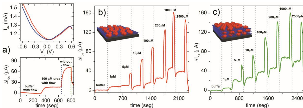
Fig. 3 (a) Transfer characteristics of a (PEI/Urease) 1 assembly in the absence (blue line) and in the presence (red line) of 100 \mu M urea (top), and the change in the channel current with and without flow (bottom). Channel current response ( \Delta I_{ds} ) monitored in real-time for (PEI/Urease) 1 (b) and (PEI/Urease) 3 (c) LbL assemblies onto rGO FETs at different concentrations of urea. The marked line indicates the elution of the next concentration of urea. Experimental conditions: 10 mM KCl and 0.1 mM HEPES at pH 6, V_g = -0.2 V and V_{ds} = 0.1 V.
