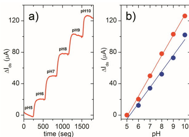
Fig. 2 (a) Change in the channel current ( \Delta I_{ds} ) of a SPS/PEI-modified rGO FET monitored in real-time varying the pH from 5 to 10 (b) \Delta I_{ds} as a function of pH for a SPS-modified rGO FET (blue circles) and a SPS/PEI-modified rGO FET (red circles). Experimental conditions: flow rate = 300 \mu\text{l/min} , V_g = -0.2 \text{ V} and V_{ds} = 0.1 \text{ V} .
