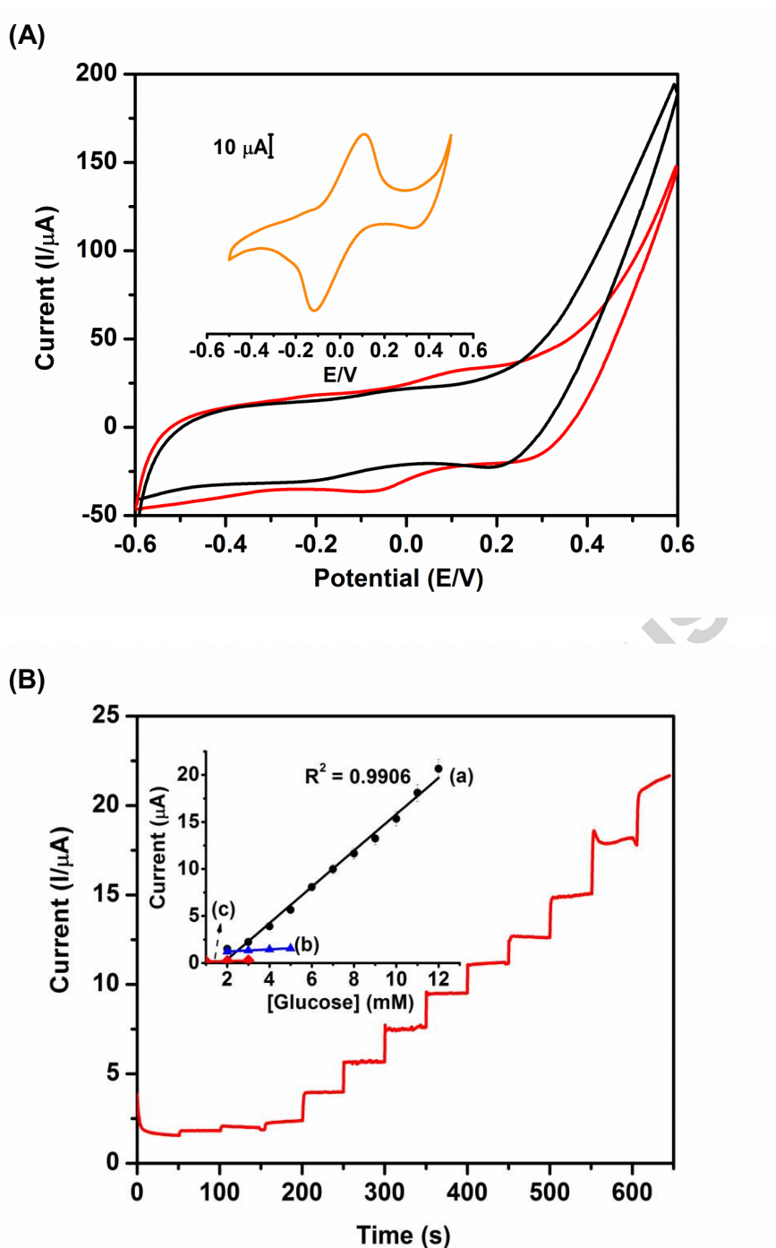
Fig. 4. (A) Cyclic voltammogram of PAA-rGO/VS-PANI/LuPc 2 /GOx-MFH (red line) 0 mM glucose and (black line) 4 mM glucose in 0.1M PBS (pH 7.0). Inset Cyclic voltammogram of PAA-rGO/VS-PANI/LuPc 2 -MFH in 0.1M PBS (pH 7.0); (B) Amperometry of PAA-rGO/VS-PANI/LuPc 2 /GOx-MFH for successive addition of glucose in 0.1M PBS (pH 7.0). Inset: calibration plot peak current versus [glucose].
