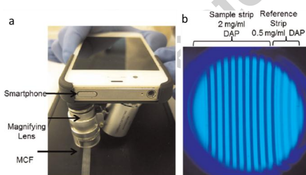
Fig. 7. (a) Magnifying lens used to read the fluorescence on a microfluidic system (b). Adapted with permission from Barbosa et al., 2015 . Copyright 2015 Elsevier.
