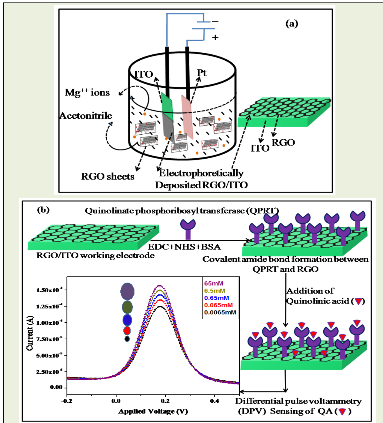
Fig. 1. Schematics for the (a) Fabrication of working electrode RGO/ITO by using electrophoretic deposition (EPD) technique and (b) immobilization of quinolinate phosphoribosyl transferase (QPRT) on working electrode RGO/ITO treated with EDC/NHS and BSA and sensing of QA via differential pulse voltammetry (DPV) technique.
