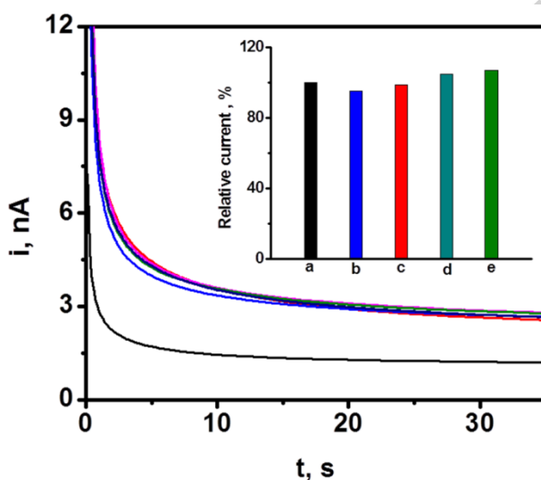
Figure 4: Chronoamperometric response of the alcohol biosensor for 20 mM alcohol followed by the addition of electroactive interferents such as AC, UA, L-Cysteine and AA, respectively (0.6 V vs. Ag/AgCl electrode). Inset shows the percentage deviation of relative current responses based on (a) 20 mM alcohol signal for 100 \mu M each of (b) AC, (c) UA and (d) L-Cysteine and 10 \mu M AA, respectively. Also shown is the blank response (black current). Conditions, as in Figure 3.
