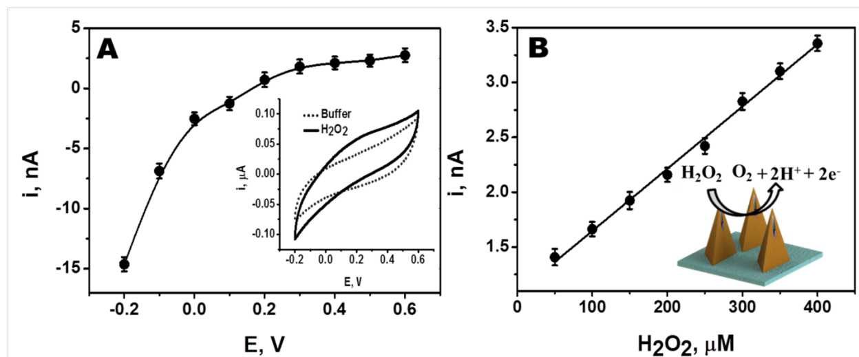
Figure 2: (A) Effect of applied potential (-0.2 V to 0.6 V) on the chronoamperometric responses of 250 \mu\text{M} H 2 O 2 measured at Pt wire integrated microneedle electrode. Also shown (inset) the corresponding cyclic voltammogram for 500 \mu\text{M} H 2 O 2 . (B) Linear chronoamperometric responses of H 2 O 2 (50 \mu\text{M} to 400 \mu\text{M} ) measured at Pt wire integrated microneedle electrode (inset shows the oxidation of H 2 O 2 on the Pt wire integrated microneedle electrode).
