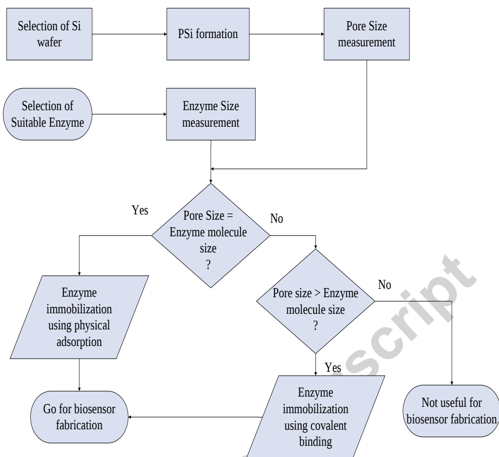
Figure 16 Flow chart for selection of pore size and porosity for enzyme immobilization
