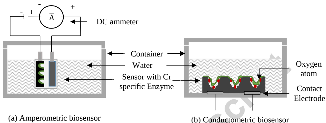
Figure 17 PS based electrochemical biosensor for Cr detection
