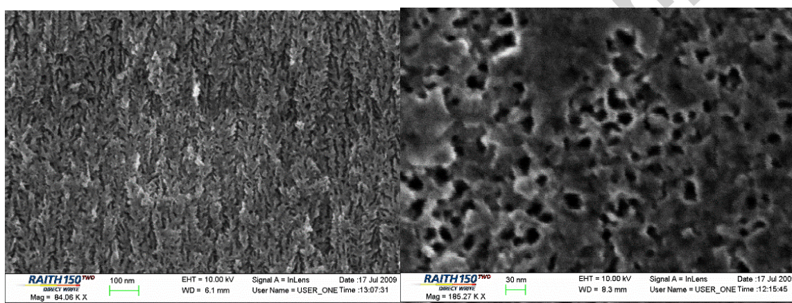
Figure 14: SEM images of a freestanding PS films fabricated using chemical anodisation of Si wafer – cross-sectional and top view respectively.
