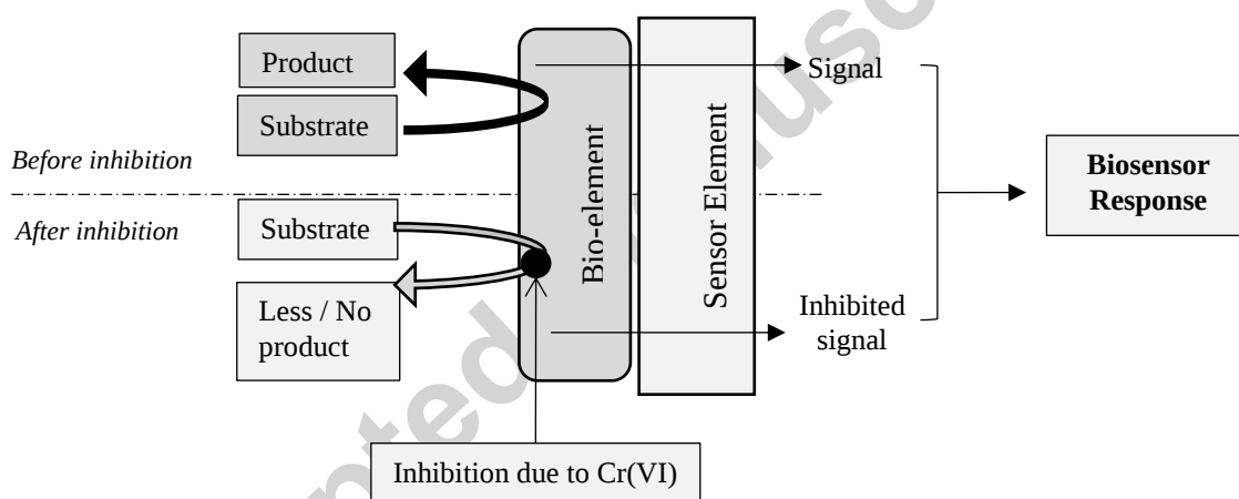
Figure 8 Working principle of enzyme inhibition-based biosensor
