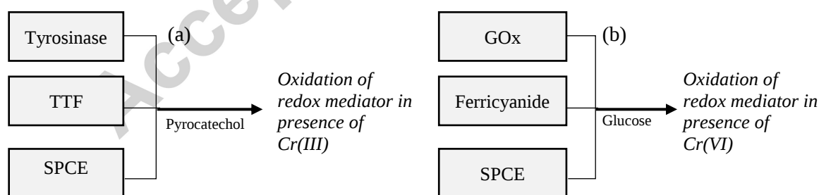
Figure 9 Enzymatic mechanism of Tyrosinase/ SPCEs and GOX/SPCEs biosensor for detection of (a) Cr(III), (b) Cr (VI)
