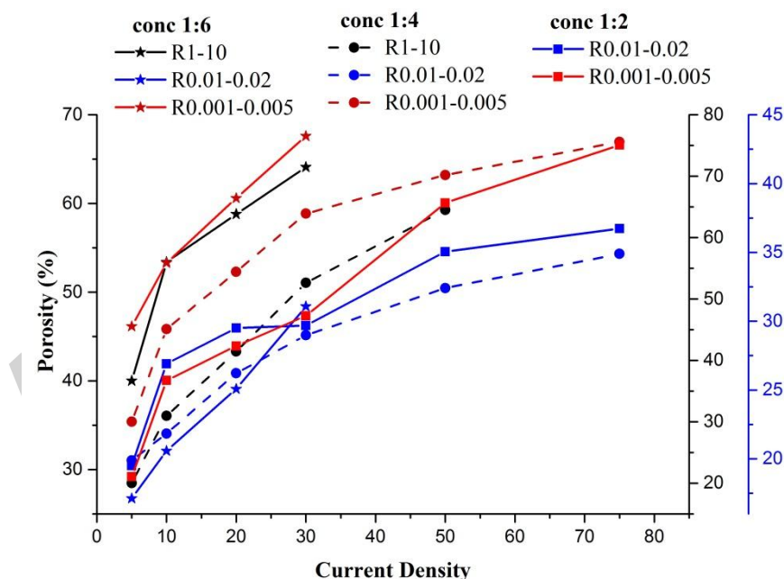
Figure 15 Effect of current density, HF concentration, and resistivity of wafer on porosity
