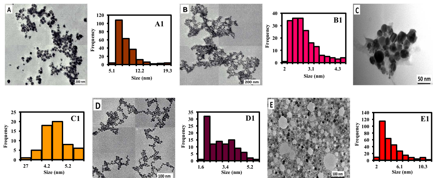
Fig. 2. TEM images and corresponding particle size distribution histograms of (A, A1) MPA-capped AgNPs, (B, B1) MPA-capped AuNPs, (C, C1) MPA-capped CS Au/AgNPs, (D, D1) MPA-capped alloyed AuAgNPs and (E, E1) Qdot646 nanocrystals.
