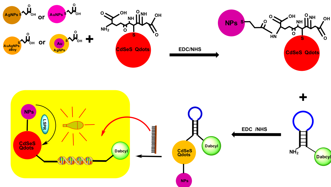
Scheme 1. The conjugation of the plasmonic NPs to GSH-CdSeS Qdots (Qdot646) to form the plasmonic NP-Qdot nanohybrids; the subsequent conjugation of the plasmonic NP-Qdots to the MB to form the plasmonic NP-Qdot-MB biosensor probe and the LSPR-mediated fluorescence signal detection of the ZIKV based on hybridization of the RNA with the DNA loop sequence of the MB.
