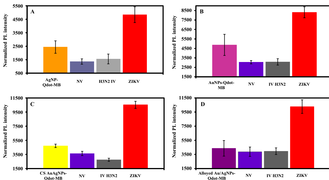
Fig. 8. Selectivity of the plasmonic NP-Qdot-MB biosensor probe toward ZIKV RNA in the presence of the negative controls (influenza virus (IV) H3N2 and norovirus (NV)). (A) AgNP-Qdot646-MB, (B) AuNP-Qdot646-MB, (C) CS Au/AgNP-Qdot646-MB and (D) alloyed AuAgNP-Qdot646-MB. Error bars represent standard deviation of 3 replicate measurements.
