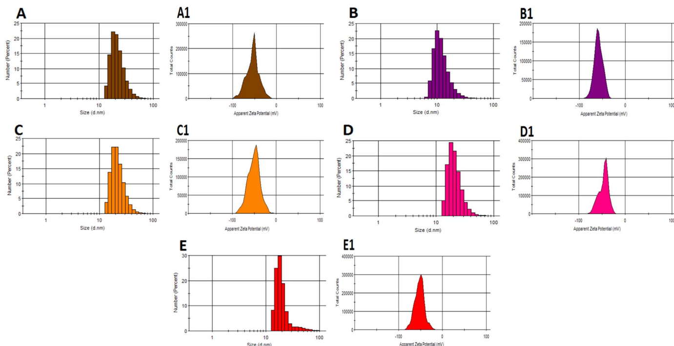
Fig. 4. DLS plot and corresponding ZP plots of (A, A1) MPA-capped AgNPs, (B, B1) MPA-capped AuNPs, (C, C1) MPA-capped CS Au/AgNPs, (D, D1) MPA-capped alloyed AuAgNPs and (E, E1) Qdot646 nanocrystals.
