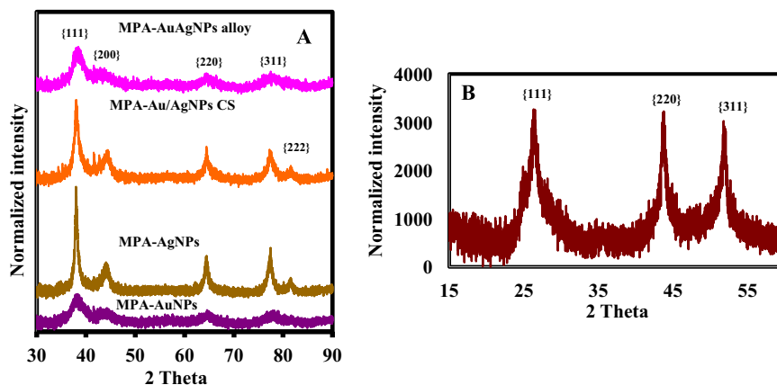
Fig. 3. PXRD spectra of the plasmonic NPs (A) and Qdot646 nanocrystals (B).
