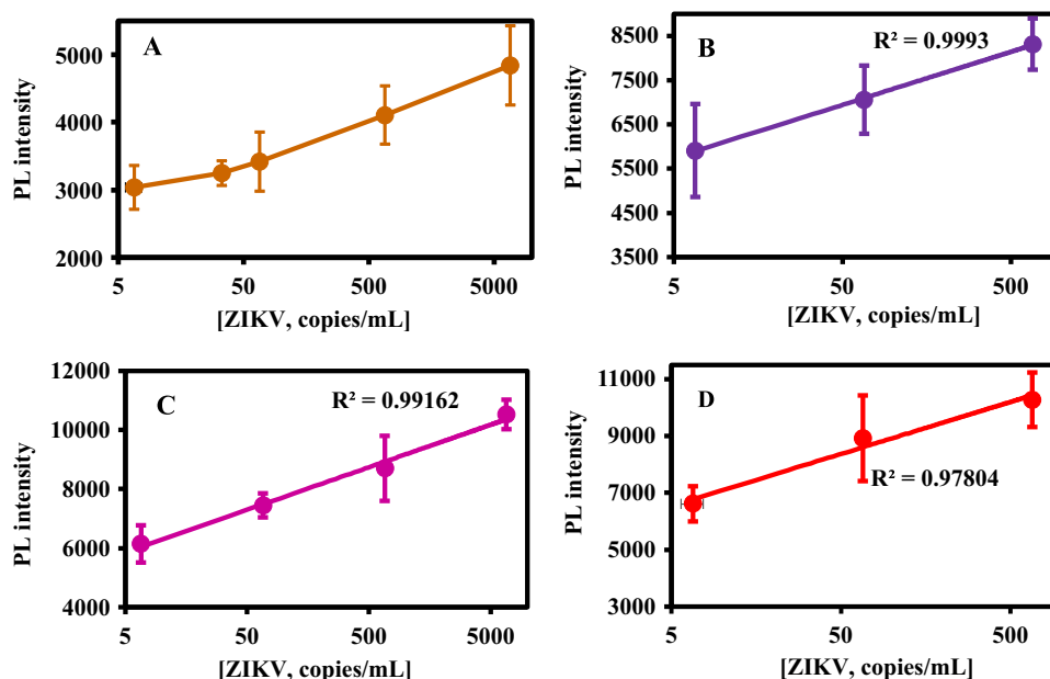
Fig. 7. Fluorescence calibration curve for ZIKV RNA detection showing the LSPR-mediated fluorescence signal of the (A) AgNP-Qdot646-MB, (B) AuNP-Qdot646-MB, (C) CS Au/AgNP-Qdot646-MB and (D) alloyed AuAgNP-Qdot646-MB. Error bars represent standard deviation of 3 replicate measurements.
