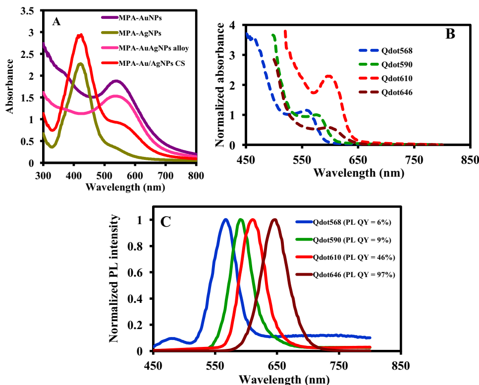
Fig. 1. UV/vis absorption spectra of the MPA-capped plasmonic NPs (A), size-dependent GSH-capped Qdots (B) and fluorescence spectra of the different-sized Qdots (C).
