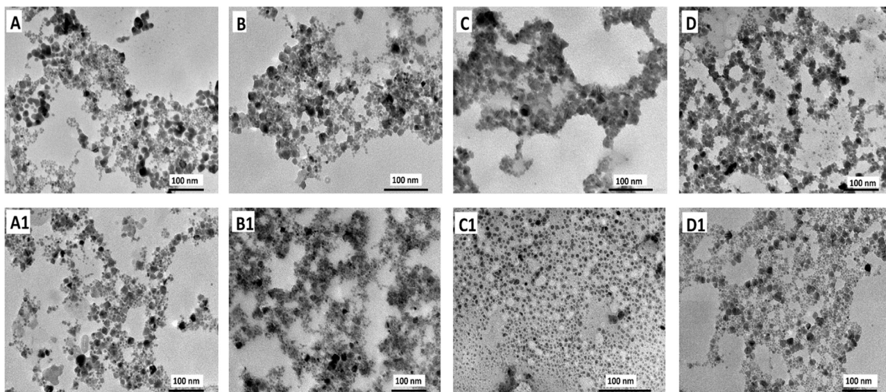
Fig. 5. TEM images of the plasmonic NP-Qdot nanohybrids: (A) AgNP-Qdot646, (B) AuNP-Qdot646, (C) CS Au/AgNP-Qdot646 and (D) alloyed AuAgNP-Qdot646; and plasmonic NP-Qdot-MB: (A1) AgNP-Qdot646-MB, (B1) AuNP-Qdot646-MB, (C1) CS Au/AgNP-Qdot646-MB and (D1) alloyed AuAgNP-Qdot646-MB.
