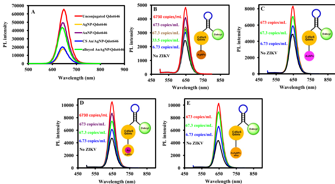
Fig. 6. (A) Fluorescence quenching effect of the plasmonic NPs on the fluorescence of Qdot646 particles. (B – E) LSPR-mediated fluorescence enhancement of ZIKV RNA using the plasmonic NP-Qdot-MB biosensor probe, (B) AgNP-Qdot646-MB, (C) AuNP-Qdot646-MB, (D) CS Au/AgNP-Qdot646-MB and (E) alloyed AuAgNP-Qdot646-MB. Inset: structure of the plasmonic NP-Qdot-MB biosensor probe.
