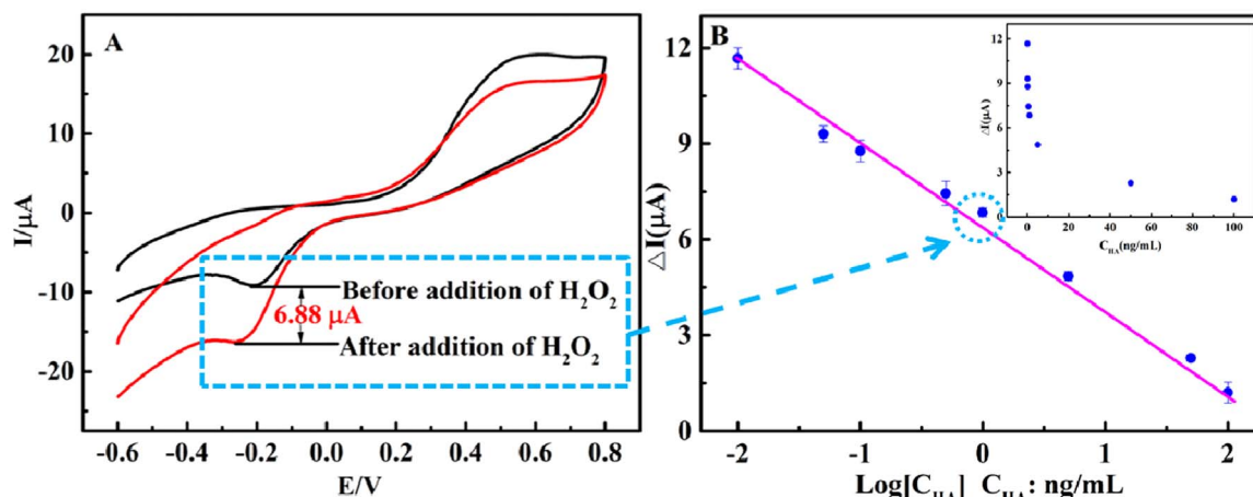
Fig. 2. A) Cyclic voltammograms; and B) calibration curve of the immunosensor and the relationship (inset in (B)) between the concentration of HA ( C_{HA} ) and the current response ( \Delta I ) of the standard solution.
