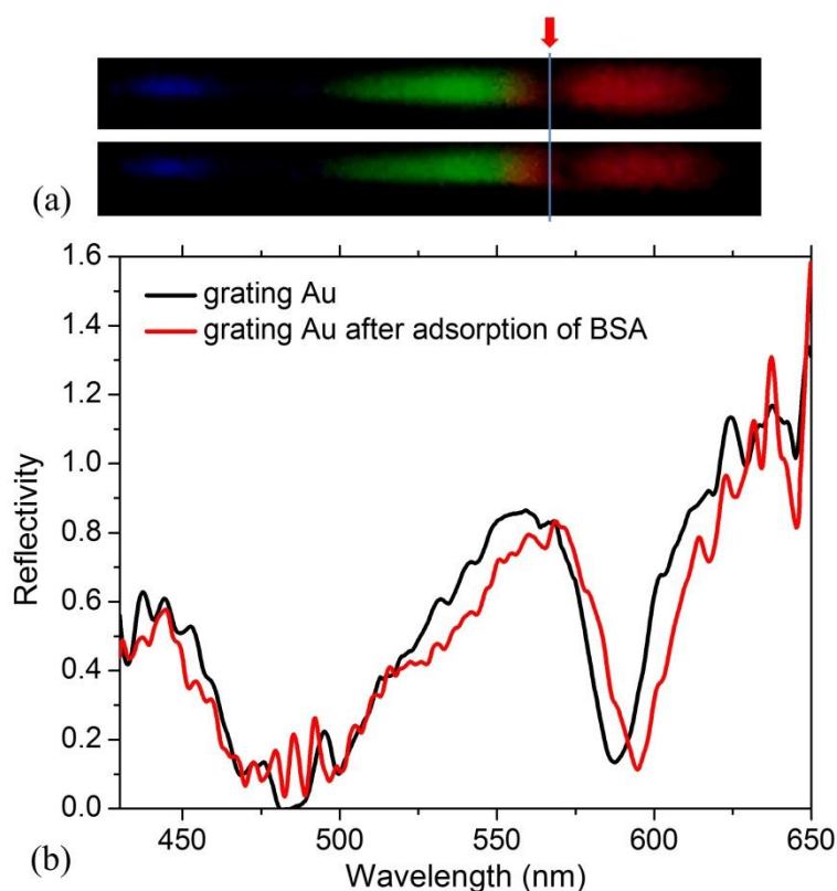
Fig. 3 (a) Color bands of grating Au before (upper one) and after incubation with 1mg/mL BSA, measured under incident angle of 5°. The line and red arrow indicate the SPR dip on the color band. (b) The corresponding SPR spectra of grating Au substrate before (black curve) and after (red curve) non-specific binding of BSA.
