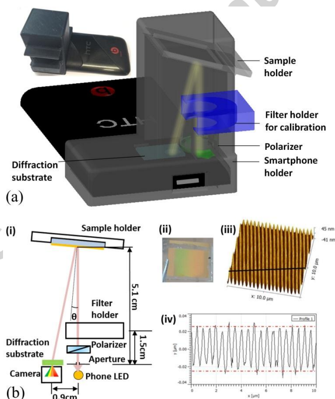
Fig. 1 (a) Schematic structure of the smartphone spectrometer relying the in-built LED light, a CD diffraction substrate and the smartphone camera. Inset is a photo of 3D printing plastic
