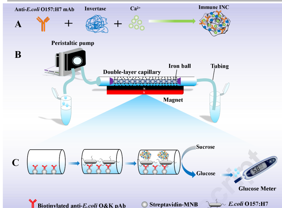
Fig.1. Schematic of this proposed biosensor using double-layer capillary based immunomagnetic separation and invertase-nanocluster based signal amplification for rapid and sensitive detection of E. coli O157:H7.
