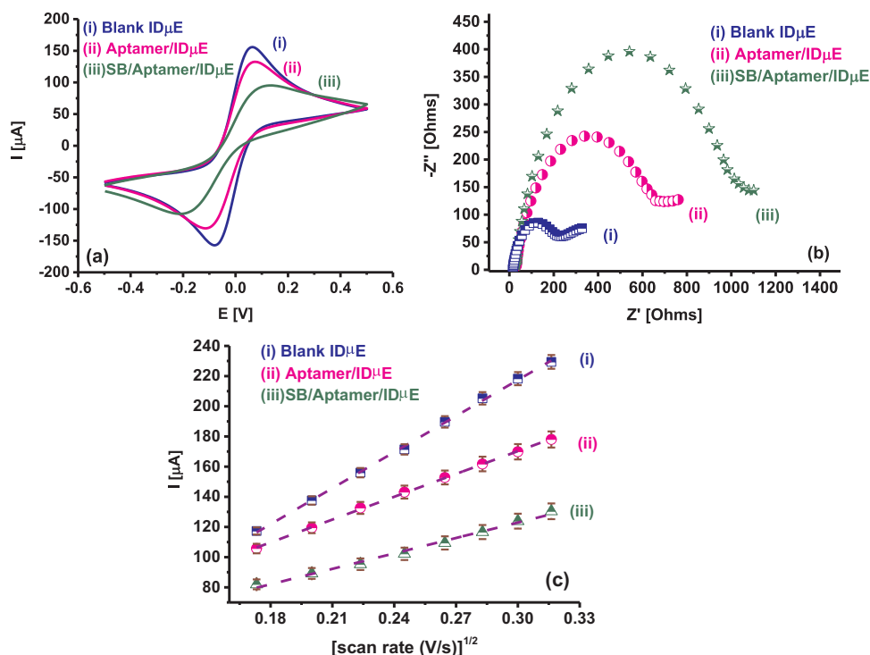
Fig. 3. Characterization of biosensor electrode fabrication at each step via (a) CV, (b) EIS and (c) scan rates study showing oxidation peak current response as a function of square root of scan rate.
