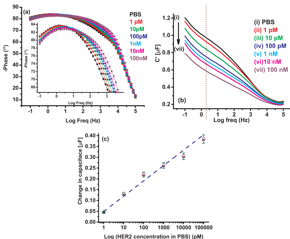
Fig. 4. (a) Phase data, (b) capacitance data for aptamer-HER2 binding on biosensor surface in PBS and (c) calibration curve using capacitance data for different concentration at 2 Hz.
