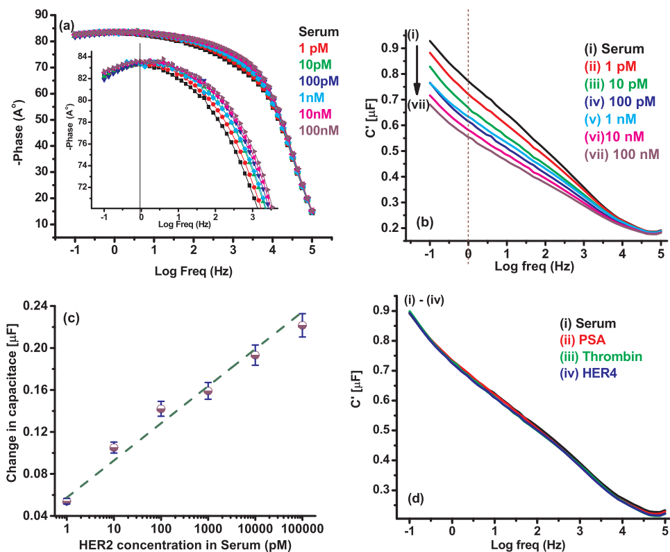
Fig. 5. (a) Phase data, (b) capacitance data for interaction between surface bound aptamer with HER2 concentrations in undiluted serum, (c) calibration curve using capacitance data for different concentration at 1 Hz, (d) capacitance data for interference study.
