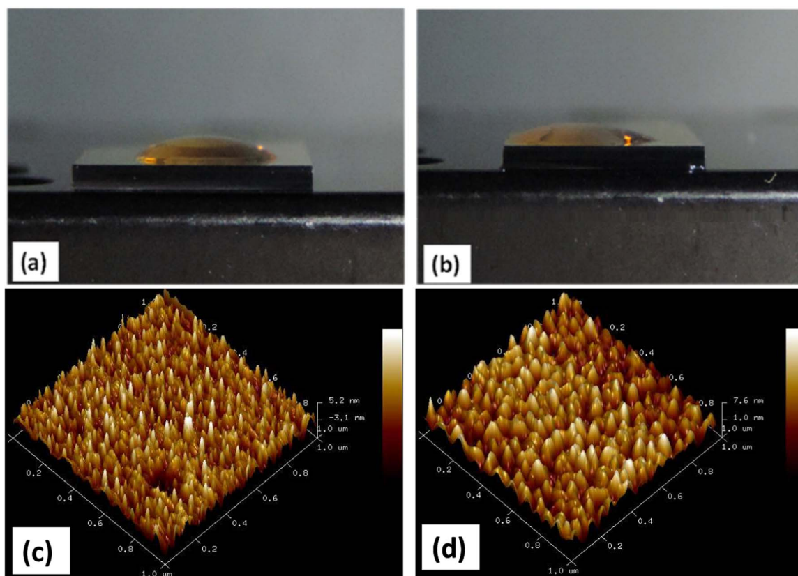
Fig. 2. Contact angle image for (a) blank cleaned gold surface, (b) after aptamer SAM formation and AFM image for (c) blank cleaned gold surface, (d) after aptamer SAM formation.
