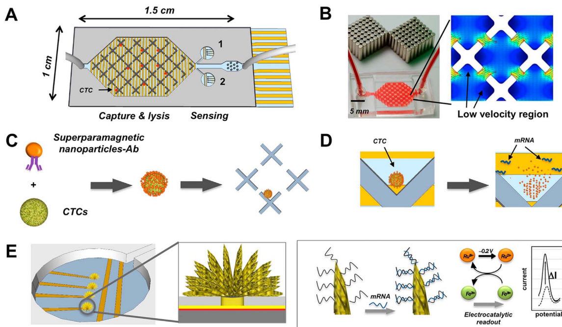
Fig. 10. The design of the sample-to-answer device for the capture and mRNA profiling of CTCs. (A) Schematic of the integrated chip featuring capture structures, electrochemical lysis electrodes, and NME sensors; (B) photographs of the fluidic capture device (left) and the flow velocity profile within the capture chamber (right); (C) selective labeling of target CTCs with antibody-functionalized MNPs and magnetically capturing the labeled cells in the vicinity of the trapping structures; (D) electrochemical lysis of the captured cells by lysis electrodes; (E) electrochemical analysis of mRNA released from the captured CTCs on the surface of PNA probe-functionalized NMEs using the [\text{Ru}(\text{NH}_3)_6]^{3+}/[\text{Fe}(\text{CN})_6]^{3-} electrocatalytic reporter system. Reprinted with permission from Mohamadi et al. (2015). Copyright 2015 American Chemical Society.
