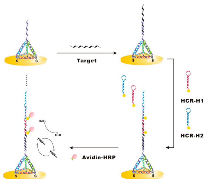
Fig. 7. Schematic illustration of the electrochemical biosensor for nucleic acid detection that takes advantage of the combined use of electrode-anchored TDNs and the HCR amplification method. Reprinted with permission from Ge et al. (2014). Copyright 2014 American Chemical Society.
