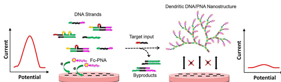
Fig. 8. Schematic illustration of the immobilization-free nucleic acid sensing strategy based on the target-induced self-assembly of dendritic DNA/PNA nanostructures. Adapted with permission from Xuan et al. (2015). Copyright 2015 American Chemical Society.
