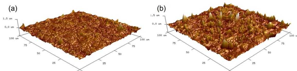
Fig. 3. AFM images of (a) ITO/poly-CzS and (b) the same surface after GOx immobilization.
