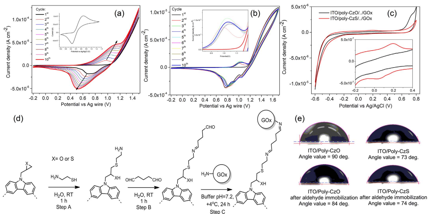
Fig. 1. Electrode modification and evaluation. Cyclic voltammogram (CV) profiles of ITO-electrode during potential cycling based electrochemical polymerization of (a) CzS and (b) CzO in DCM 0.1 M of NaBu 4 PF 6 at scan rate of 50 mV s -1 , 1st to 10th cycle (Inset: CV of ferrocene as external standard), (c) CVs of ITO/poly-CzO and poly-CzS/amine/aldehyde/GOx in buffer, pH 4.0, (Inset: increased spectral range from -0.2 to +0.4 V), (d) schematic representation of step-by-step self-assembly-based immobilization of GOx on ITO/poly-CzO and ITO/poly-CzS electrodes, (e) water contact angle measurements of ITO/poly-CzO(S) electrode before and after the treatment with glutaraldehyde.
