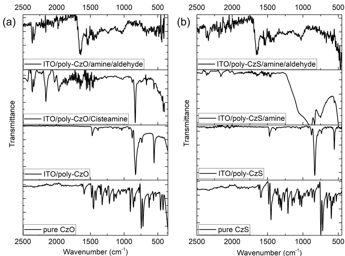
Fig. 2. ATR-IR spectra of (a) pure CzO and (b) pure CzS, both deposited on ITO/poly-CzO(S), ITO/poly-CzO(S)/amine, ITO/poly-CzO(S)/amine/aldehyde.
