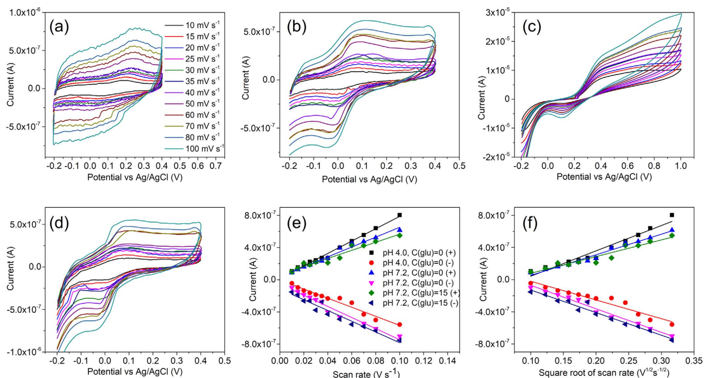
Fig. 4. (a) CVs at different scan rates when pH 4.0 and C(glu) = 0, (b) pH 7.2 and C(glu) = 0, (c) pH 4.0 and C(glu) = 15 mM, (d) pH 7.2 and C(glu) = 15 mM, (e) current vs scan rate and (f) current vs square root of scan rate and the corresponding fitting lines. Scan rates in the range from 10 to 100 \text{mV s}^{-1} were used for all CV experiments.
