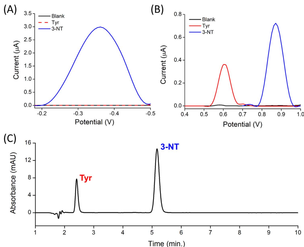
Fig. 3. Discrimination of Tyr and 3-NT via (A) reduction and (B) oxidation signals with voltammetry, and (C) HPLC.
