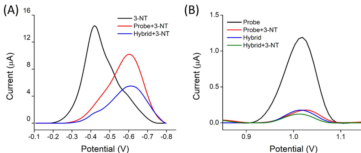
Fig. 6. Voltammograms of reduction signals of (A) 3-NT and (B) oxidation signals of guanine obtained from probe and hybrid coated PGEs. The experimental conditions are: PGEs pretreatment, 1.4 V for 30 s without stirring in ACB, 5 µg/mL probe immobilization for 20 min, interaction with 7 µg/mL target for 45 min, rinsing with PBS, interaction with 3-NT for 10 min and DPV measurement by scanning between -0.1 V and -0.8 V for reduction, and +0.7 and +1.1 V for oxidation in ACB.
