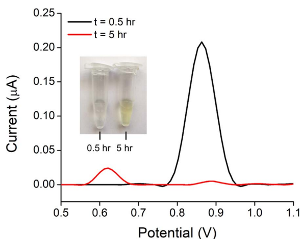
Fig. 5. Voltammogram of oxidation signals for 15 µg/mL 3-NT measured in PBS after the preparation of the solution 0.5 h. and 5 h.
