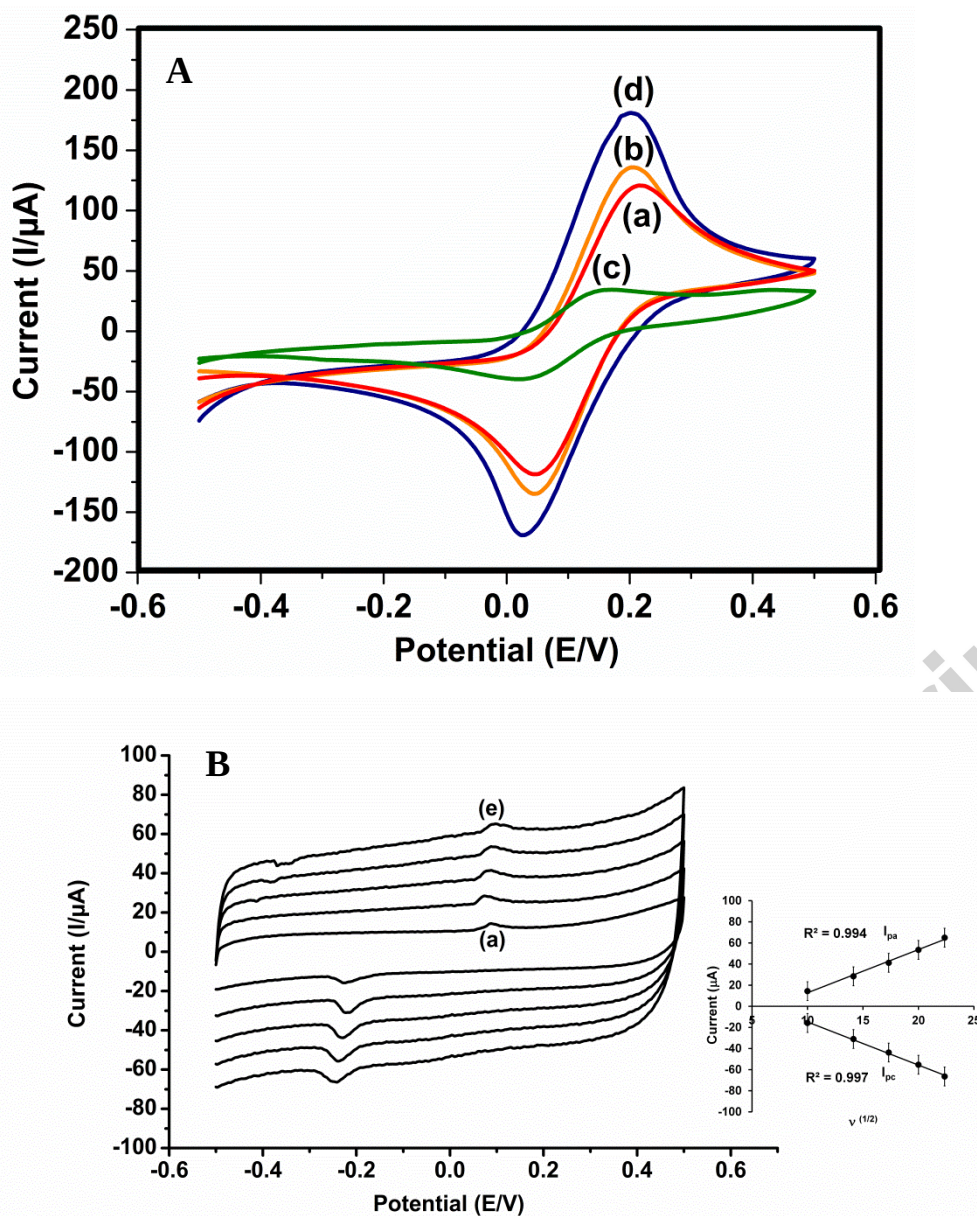
Fig. 3 (A) Cyclic voltammogram of (a) \text{SiO}_2 , (b) \text{SiO}_2(\text{LuPc}_2) , (c) PANI(PVIA), (d) \text{SiO}_2(\text{LuPc}_2) -PANI(PVIA)-CNB recorded in 5 mM Potassium ferro/ferricyanide solution containing 0.1 M NaCl; scan rate = 100 mV/s (B) Cyclic voltammogram of \text{SiO}_2(\text{LuPc}_2) -PANI(PVIA)/GOx-CNB in \text{N}_2 saturated 0.1 M PBS (pH 7.0) containing 0.1 M NaCl for different scan rate 100-500 mV/s (a-e); inset: plot of v^{1/2} vs I_p
