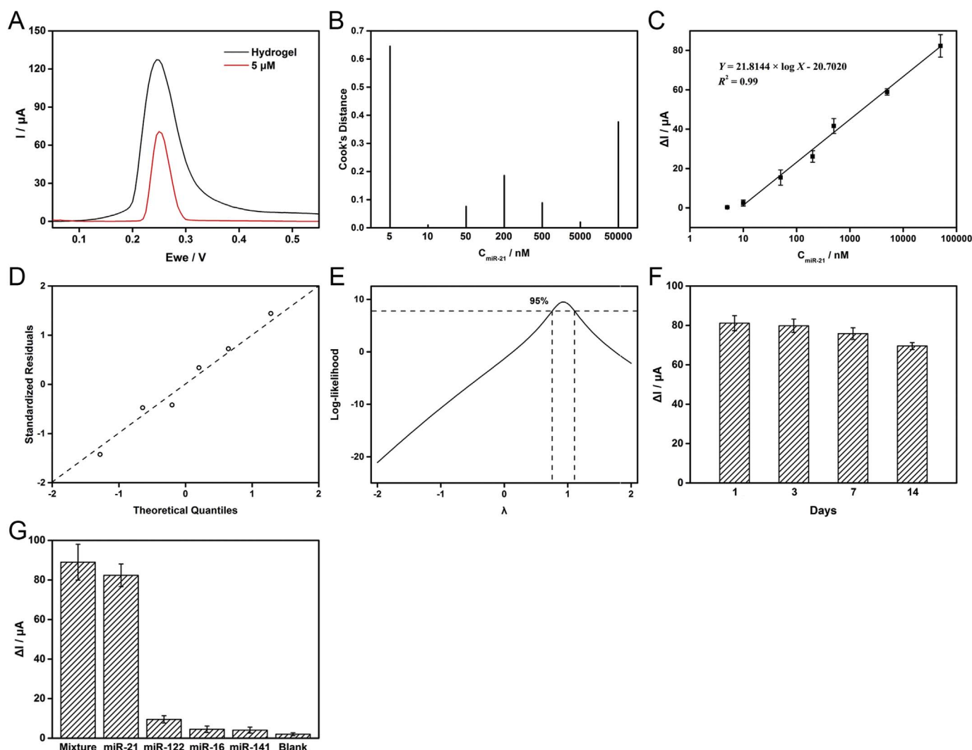
Fig. 3. (A) DPV for the electrochemical DNA hydrogel in the presence of target miR-21 at 5 \mu M . (B) Data point of 5 nM is an apparent outlier identified from Cook's distance plot, indicating detection of 5 nM does not strictly follow the linearity relationship between \Delta I and miR-21 concentration. (C) Linear regression model between \Delta I and miR-21 concentration for the electrochemical DNA hydrogel biosensor. (D) Residual of each data point in the normal Q-Q plot is uniformly distributed along a straight line, which means the standardized residuals accord with the normal distribution. (E) The corresponding abscissa of the vertex of parabola is close to 1, indicating no data transformation required in the model. (F) The storage stability of the hydrogel biosensor. (G) The selectivity and specificity of the hydrogel biosensor with different interferences: miR-21 (50 \mu M ), miR-122 (50 \mu M ), miR-16 (50 \mu M ), miR-141 (50 \mu M ), and a mixture solution (50 \mu M of miR-21 and 500 \mu M of each interference).
