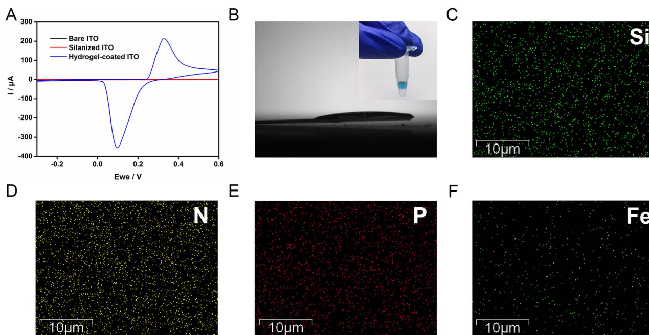
Fig. 2. (A) CV curves of bare, silanized, and hydrogel-coated ITO electrodes in PBS. (B) Images of contact angle test for ITO electrode immobilized with DNA hydrogel, inserted with visual observation of DNA hydrogel and dyeing solution stratification. EDS phase distribution images of silanized ITO electrode for the analysis of Si (C) and hydrogel-coated ITO electrode for the analysis of (D) N, (E) P and (F) Fe. Bright spots represent the locations of the EDS analysis points. Scale bar is 10 \mu m.
