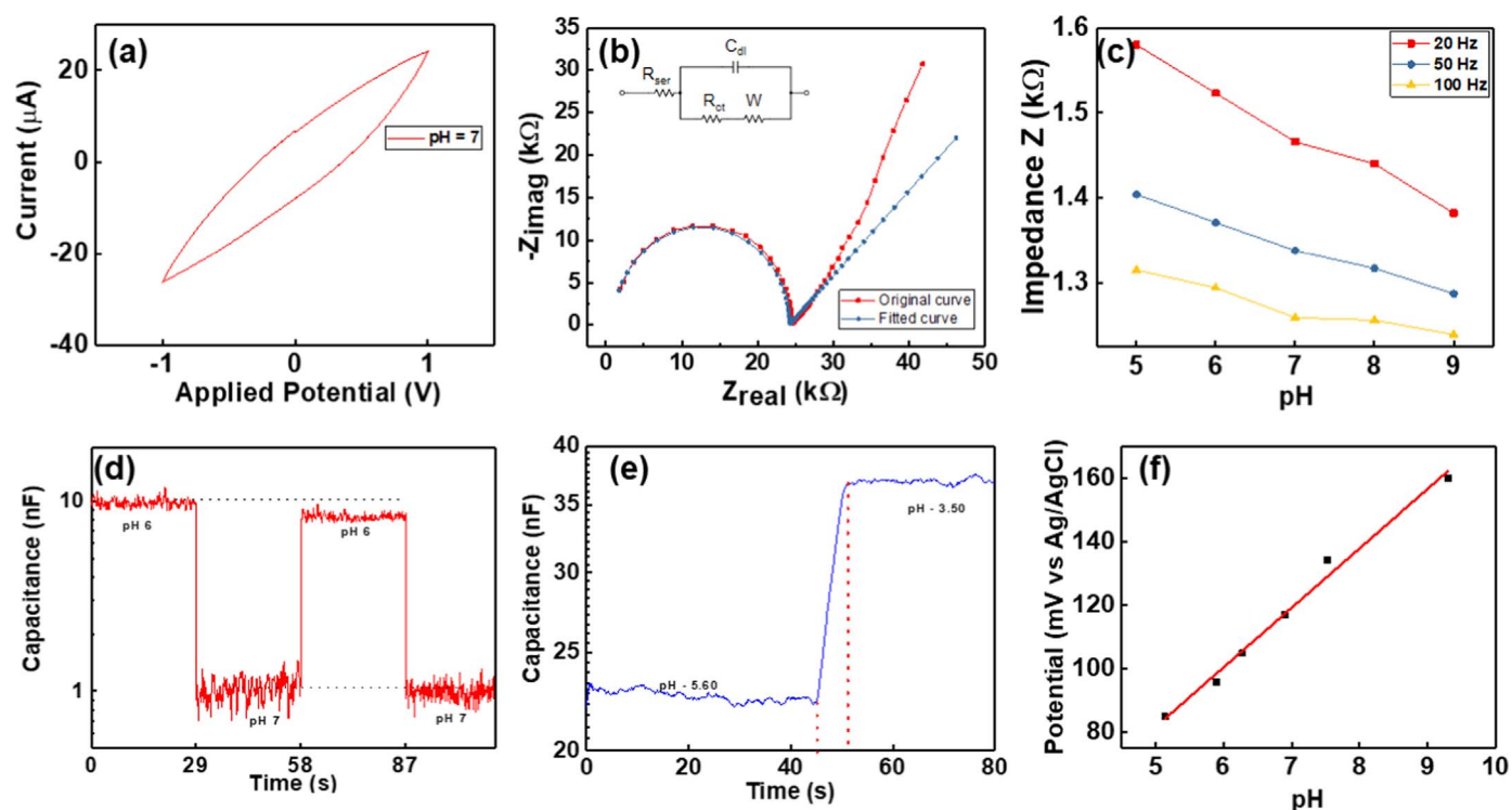
Fig. 3. (a) CV curve and (b) Nyquist plot for graphite-polyurethane composite electrode at pH 7 buffer solution and fitted curve based on Randles circuit model (c) impedance versus pH measured between SE and RE at selected frequencies (d) hysteresis in pH response and (e) response time of the sensor (f) potentiometric performance of the pH sensor.
