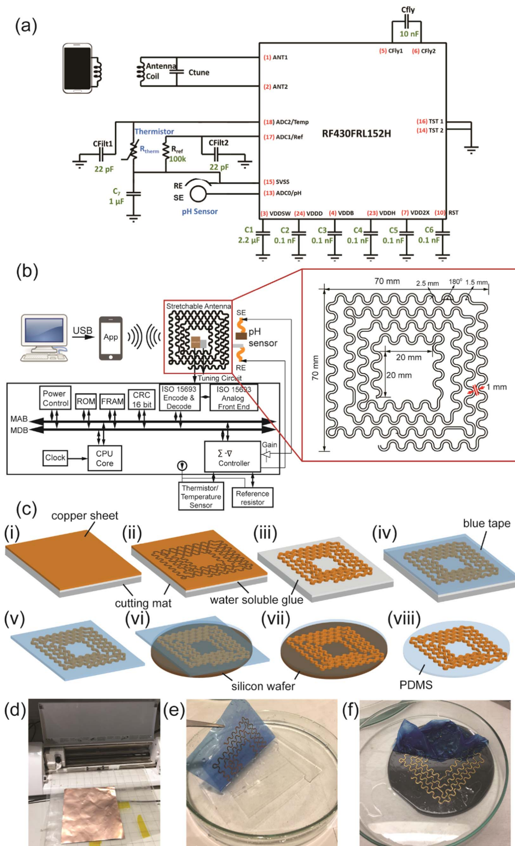
Fig. 2. (a) Circuit design and (b) system-level block diagram for wireless pH data transmission with the inset image of antenna design and (c) Fabrication steps of stretchable antenna including (i) laminating flexible copper sheet to cutting mat with water-soluble glue as sacrificial layer, (ii) blade cutting the antenna pattern, (iii) removing the rest of material, (iv) attaching the blue tape over the antenna pattern, (v) dissolving the glue in water and transferring the antenna pattern to blue tape, (vi) adhering to partially cured PDMS substrate (separately prepared through spin-coating on silicon wafer), (vii) curing PDMS and dissolving blue tape in acetone and (viii) detaching the PDMS substrate from silicon wafer. Photos of critical steps c(i), c(v) and c(vii) are also included in (d), (e) and (f) respectively.
