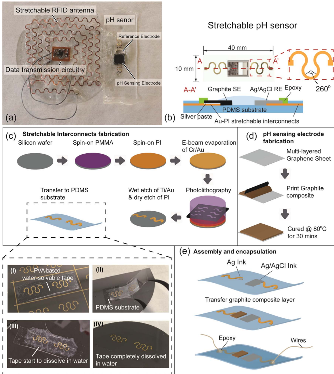
Fig. 1. (a) Photo of stretchable wireless system for sweat pH monitoring, (b) Schematic diagram of stretchable pH sensor with graphite-polyurethane composite SE, Ag/AgCl-based RE and a pair of stretchable interconnects. Schematic diagram of the fabrication process for (c) stretchable interconnects, (d) SE electrodes (e) assembly and encapsulation of sensor patch.
