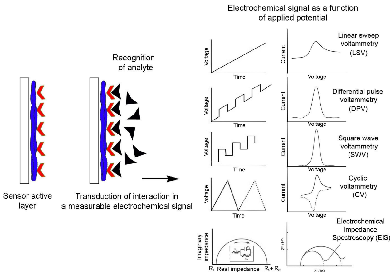
Figure 1. Schematic representation of an electrochemical sensor, its interaction with the analyte, and the transduction of these interactions into measurable signals
