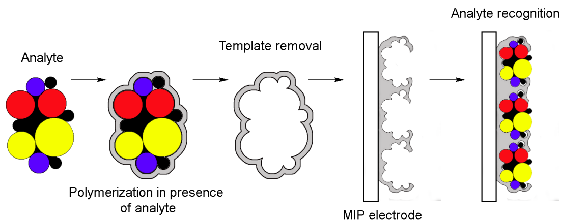
Figure 2. Schematic representation of a molecularly imprinted polymer (MIP) electrode
