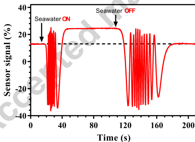
Figure 5. Sensor signal response to the flow of seawater.
