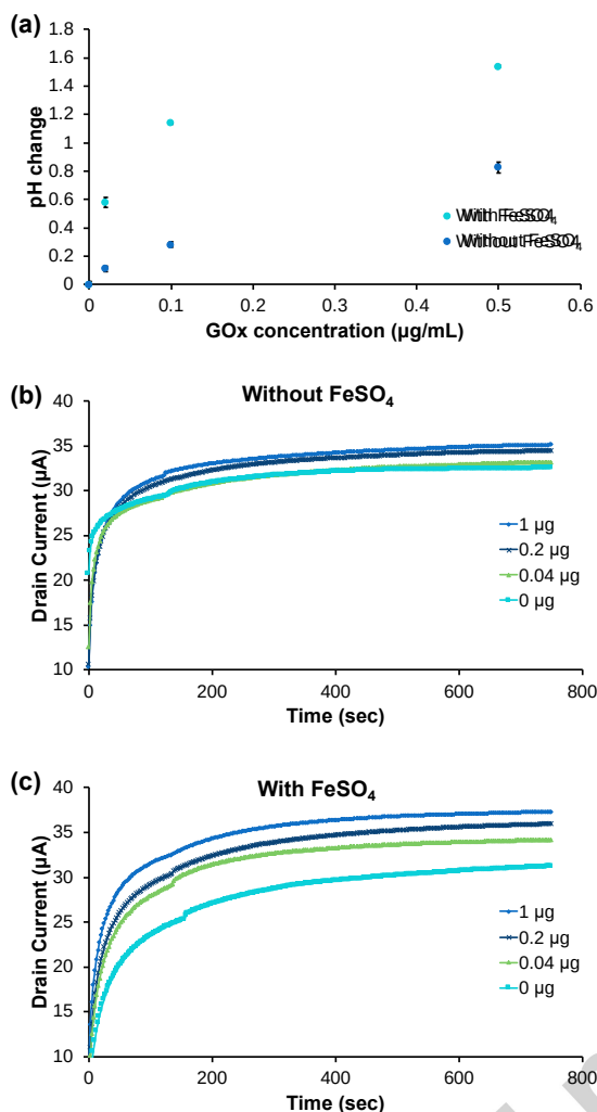
Fig. 4. Enhancement in proton generation by \text{FeSO}_4 . (a) Adding \text{FeSO}_4 can increase proton generation with the same concentration of GOx. (b) Real-time measurement of proton generation with various GOx concentrations over 750 seconds (b) without and (c) with \text{FeSO}_4 in the reaction solution over a 750 second period.
