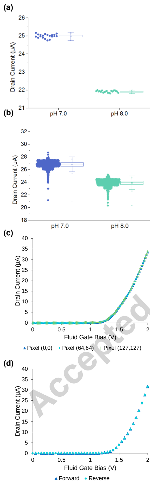
Fig. 3. Accuracy and repeatability of DG-ISFET chip. (a) Current responses of 20 repeated measurements of pH 7 and pH 8 standard buffers using the DG-ISFET chip.
