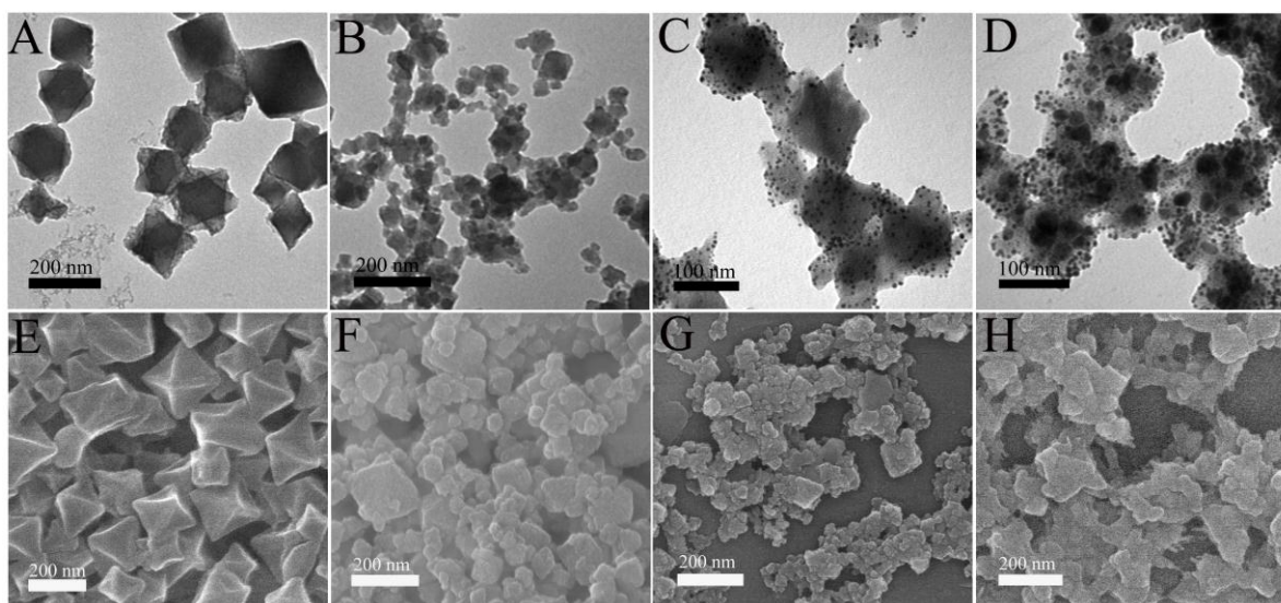
Fig. 1. TEM images of (A) \text{NH}_2\text{-MIL} , (B) Hemin-MIL, (C) Au-Hemin-MIL, (D) pDNA-Au-Hemin-MIL-DNAzyme. SEM images of (E) \text{NH}_2\text{-MIL} , (F) Hemin-MIL, (G) Au-Hemin-MIL, (H) pDNA-Au-Hemin-MIL-DNAzyme.
