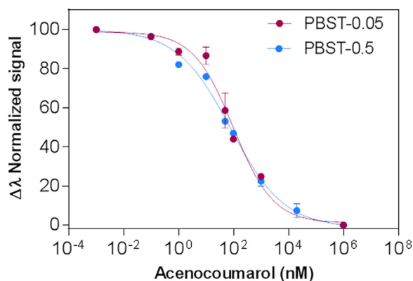
Fig. 3. Standard calibration curves of acenocoumarol immunoassay in PBST-0.5 and PBST-0.05. Each point represents the mean \pm SD of duplicates.
