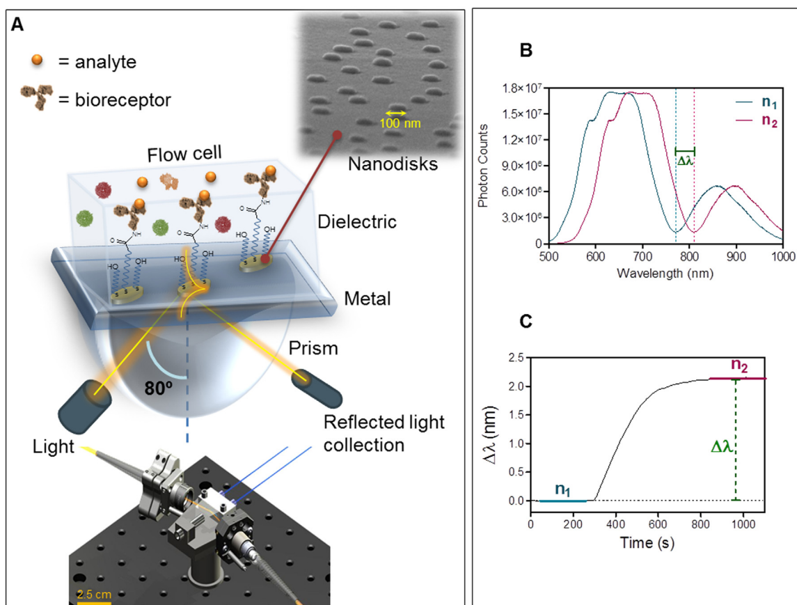
Fig. 1. (A) Schematic representation of the nanoplasmonic biosensor. (B) Graph showing the displacement of the resonance peak ( \lambda_{LSPR} ) to RI changes (photon vs. \lambda (nm)). (C) Real time monitoring of wavelength displacements ( \Delta\lambda vs. time (s)).
