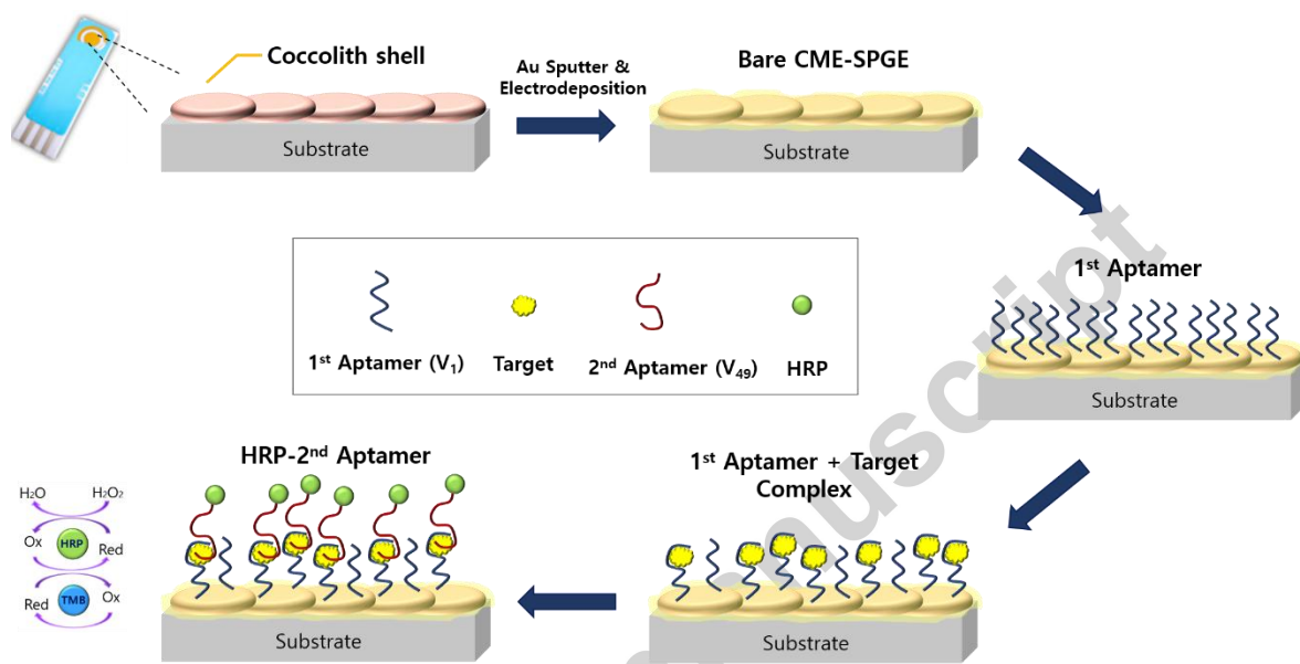
Scheme 1. Schematic illustration of the preparation of the coccolith modified electrodeposited on the screen-printed gold electrode (CME-SPGE) and a cognate pair of aptamer-based sandwich-type electrochemical aptasensor.
