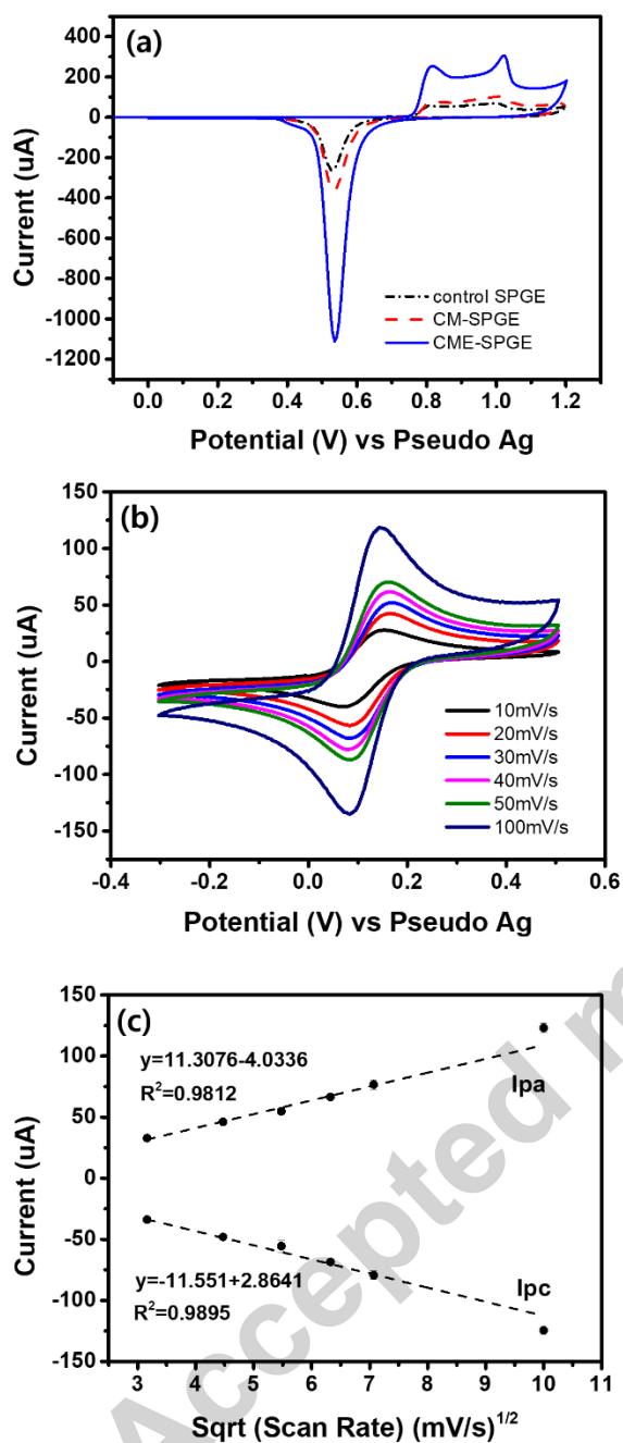
Fig. 2. Cyclic voltammograms of (a) control screen-printed gold electrode (bare SPGE), the coccolith modified screen-printed gold electrode (CM-SPGE), and the coccolith modified electrodeposited screen-printed gold electrode (CME-SPGE), respectively, obtained at 100 \text{ mVs}^{-1} in 0.5 \text{ M H}_2\text{SO}_4 solution; (b) Cyclic voltammograms of CME-SPGE at various scan rates from 10 to 100 \text{ mVs}^{-1} in 5 \text{ mM K}_3[\text{Fe}(\text{CN})_6] solution containing 0.1 \text{ M KCl} . (c) Plots of Anodic peak current ( I_{pa} ) and Cathodic peak current ( I_{pc} ) versus square root of scan rates.
