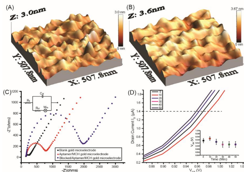
Fig. 1. AFM characterization of bare ID \mu E (A) and protein /aptamer- ID \mu E surfaces (B) (scanned area \sim 0.5 \times 0.5 \mu\text{m}^2 ). (C) EIS characterization of blank and modified ID \mu Es. (D) AptaFET stability studies in binding buffer from the plot of drain current ( I_D ) versus gate voltage ( V_{GS} ) at different incubation time. Inset plot depicts gate voltage at fixed drain current verses different incubation time.
