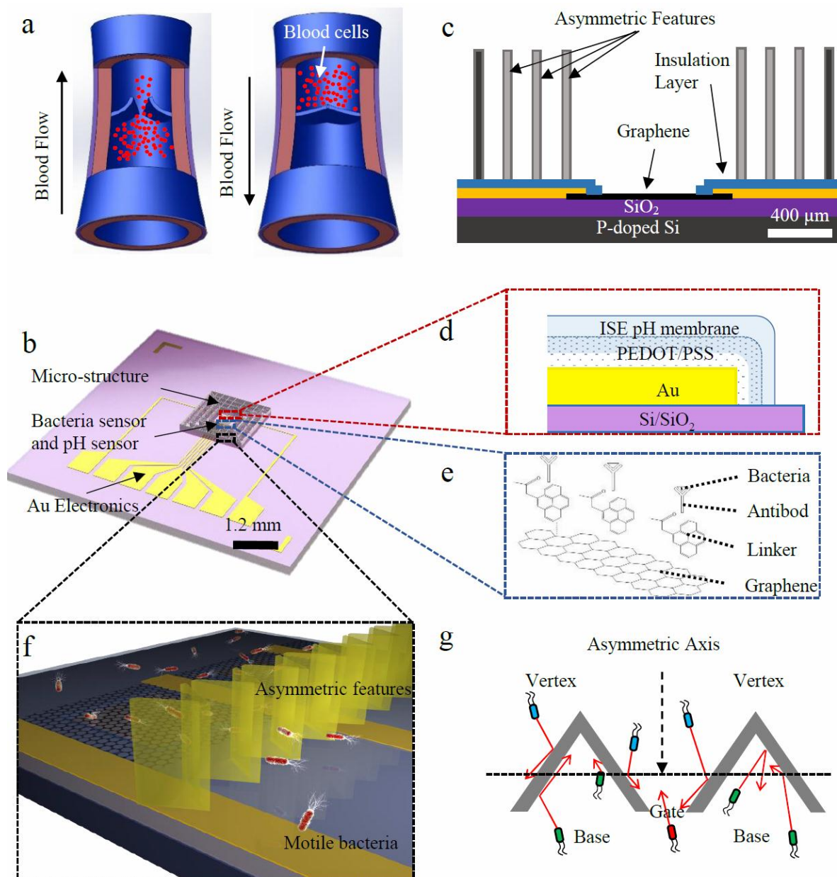
Figure 1. Layout illustration of bio-inspired 3D micro-structure enhanced graphene sensor. (a) Schematic diagram of the venous valves in blood vein. (b) 3D view of the sensor on \text{SiO}_2/\text{Si} substrate. (c) Cross-section of the graphene bacteria sensor. (d) Cross-section of pH sensor and (e) chemical functionalisation of bacteria sensor. (f) 3D view of concentrating mechanism. (g) Top view of the asymmetric features and 2D concentrating mechanism.
