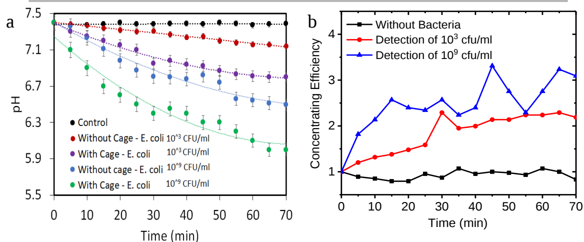
Figure 4. pH analysis of 3D micro-structure enhanced graphene bacteria sensor (a) Comparison of the response to pH from bacteria culture without and with a micro-structure towards the detection of 10^3 and 10^9 cfu/ml concentration. (b) Concentrating efficiency vs time for the detection of 10^3 and 10^9 cfu/ml E. coli . Detection towards blank buffer is shown as control.
