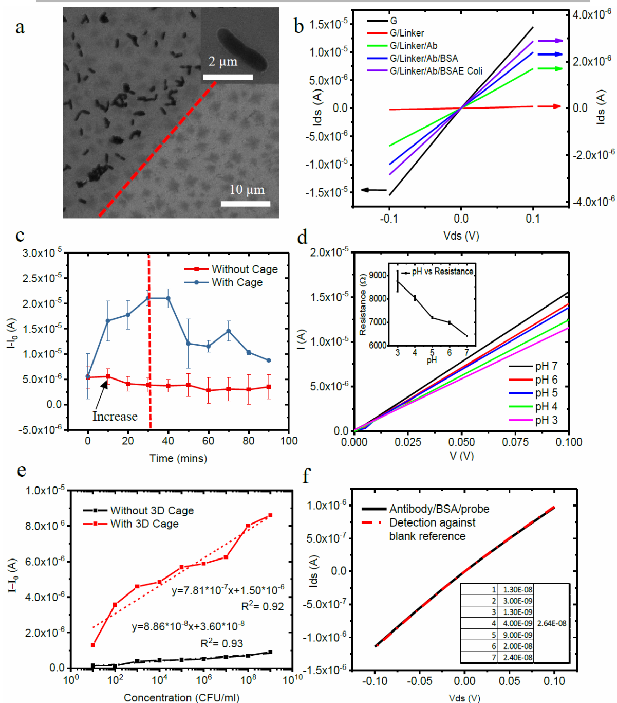
Figure 5. Electrical analysis of 3D micro-structure enhanced bacteria sensing performance. (a) Control experiment of cell bonding on the functionalised and the non-functionalised graphene. Inset: individual E. coli immobilised on the functionalised graphene. (b) Transfer curves of one graphene sensing window after functionalization. (c) Electrical current vs time for the detection of E. coli in culture medium. (d) Electrical signal vs standard pH references. (e) Electrical detection of different cell concentrations from the devices with/without the 3D
