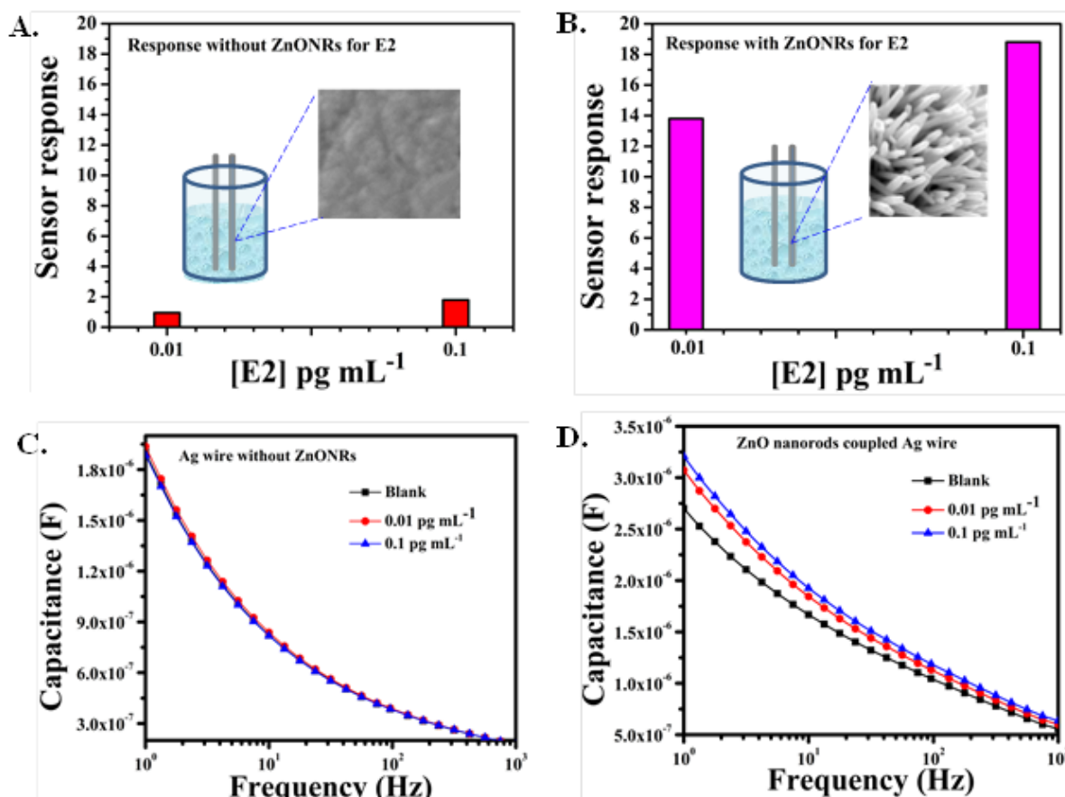
Figure 3: A. Sensor response of Ag-mAb-E2 B. Sensor response of Ag-ZnONRs-mAb-E2 C. Capacitance spectra of the Ag-mAb-E2 immunosensor D. Capacitance spectra of the Ag-ZnONRs-mAb-E2.
