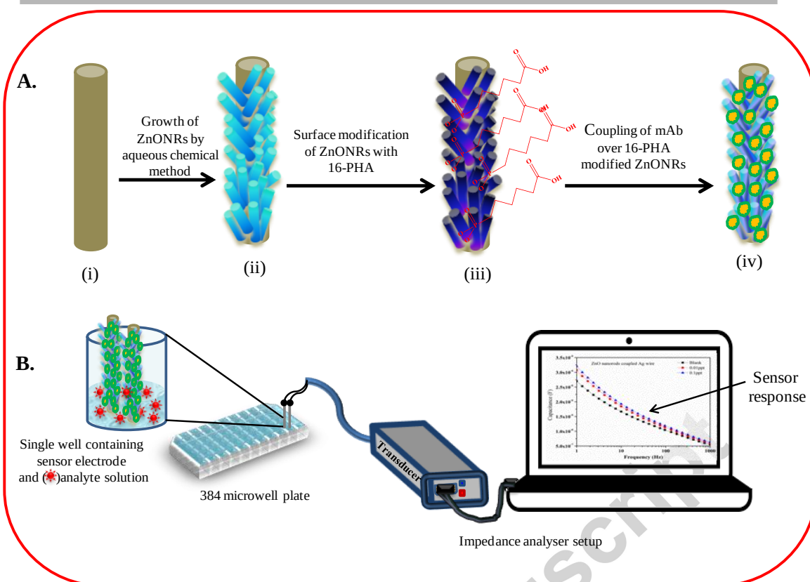
Scheme 1: Schematic representation of nanoimmunosensor construction; A. Preparation of ZnONRs-E2 probe (i) Ag wire electrode (ii) ZnONRs grown on Ag wire electrode (iii) Self assembly of 16-PHA on Ag-ZnONRs (iv) mAb-E2 functionalized Ag-ZnONRs B. EIS measurement setup comprising a pair of Ag-ZnONRs-mAb-E2 in 384 well format connected via impedance analyser.
