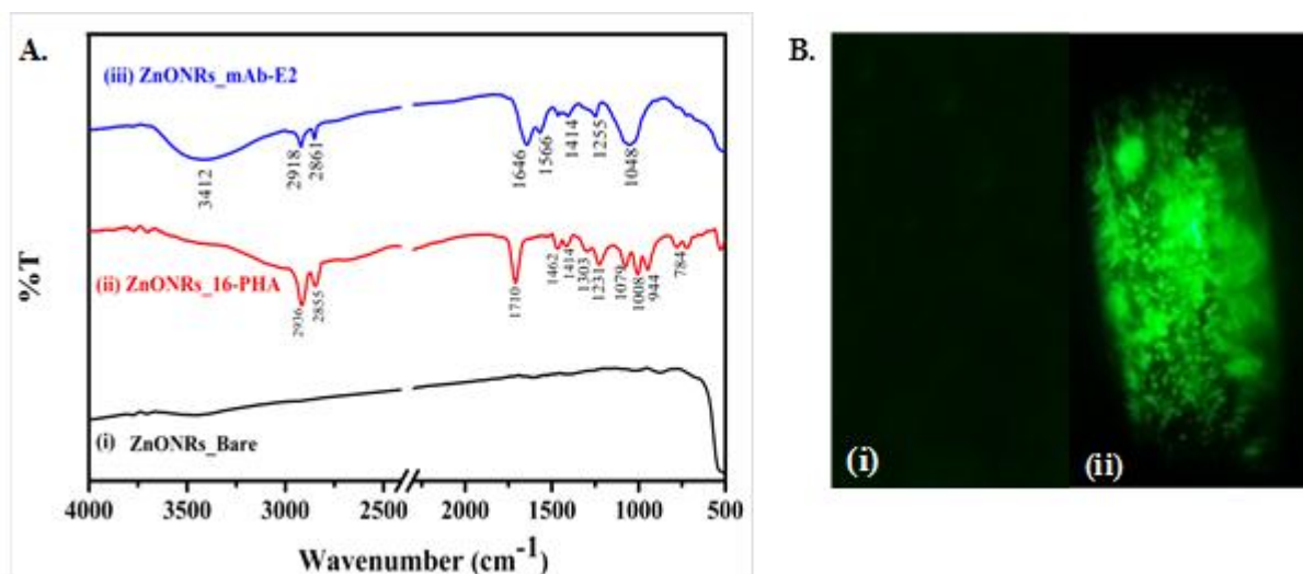
Figure 1: A. Step wise surface characterization of sensing probe using FTIR in ATR mode at 64\text{ cm}^{-1} resolution (i) bare Ag-ZnONRs (ii) 16-PHA functionalized Ag-ZnONRs and (iii) binding of mAb-E2 on Ag-ZnONRs; B. Fluorescence microscopic image (i) bare Ag-ZnONRs (ii) 2° FITC labeled antibody bound to Ag-ZnONRs-mAb-E2.
