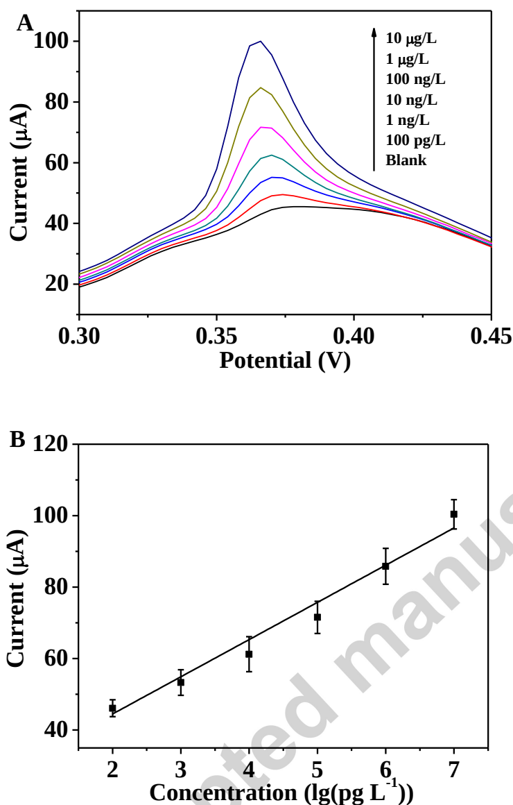
Fig 4. (A) Differential pulse voltammograms of the PP-AuNP-Ap/Au biosensor at concentrations of PCB77 ranging from 100 pg L -1 to 10 µg L -1 . Pulse amplitude, 50 mV. (B) The increase in the peak current for different concentrations of PCB77. The standard deviations are all less than 5%.
