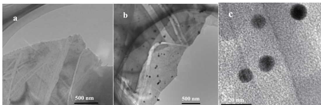
Fig 1. TEM images of (a) PP and (b) the PP-AuNP nanocomposite and (c) an enlarged image of the PP-AuNP nanocomposite.
