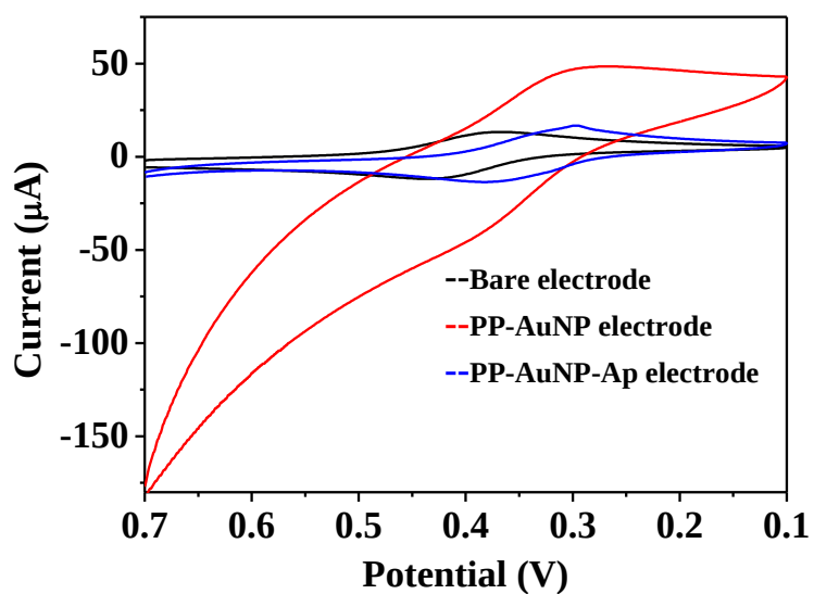
Fig 3. Cyclic voltammograms of the different Au electrodes in 5 mmol L -1 [Fe(CN) 6 ] 3-/4- . (a) Bare Au electrode (black line), (b) PP-AuNP/Au electrode (red line) and (c) PP-AuNP-Ap/Au electrode (blue line).
