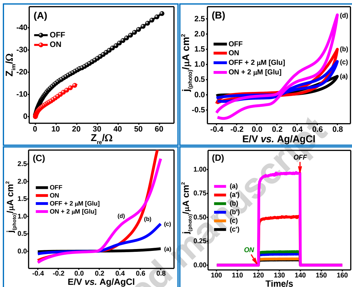
Fig. 3 (A) Electrochemical impedance spectroscopy (Nyquist plots); (B) Cyclic voltammograms and (C) Linear sweep voltammograms were obtained at GODx/NDC-TiO 2 NPs/ITO electrode in the (a, b) absence and (c, d) presence of 2 \mu M of glucose with (a, c) light OFF and (b, d) ON. (D) The j_{(photo)} - t responses of GODx/NDC-TiO 2 NPs/ITO (a, a'); GODx/TiO 2 NPs/ITO (b, b') and GODx/NDC/ITO (c, c') electrodes in the presence (a, b, c) and absence (a', b', c') of 2 \mu M of Glu in 0.1 M pH 7.0 PBS at 0.40 V vs. Ag/AgCl.
