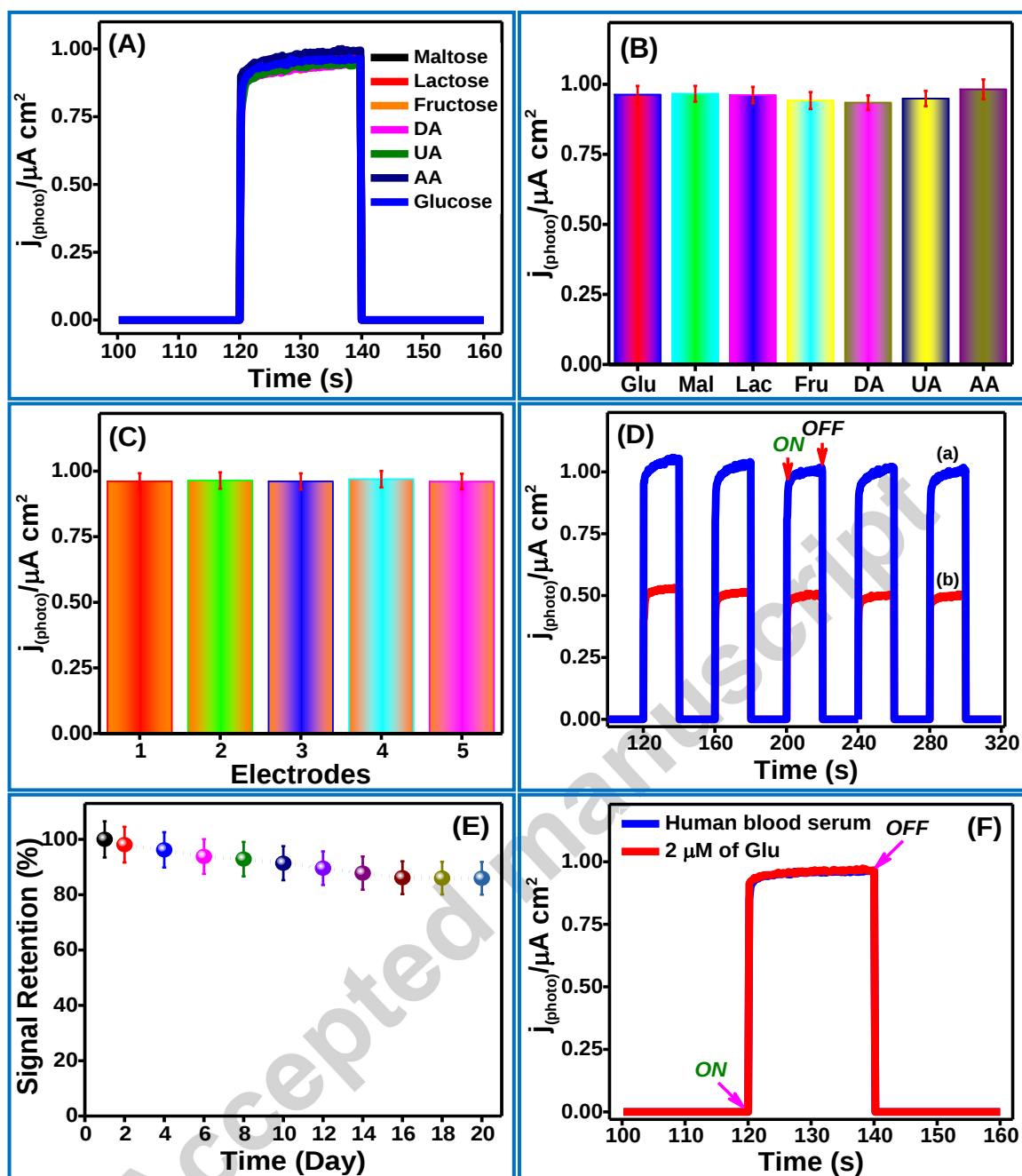
Fig. 5 (A, B) Effect of interferences on the response photocurrents. Experiments were performed in 0.1 M PBS (pH 7.0) containing 2 \mu M of Glu with maltose, lactose, fructose, DA, UA and AA with light ON. (C) Reproducibility on five parallel prepared GODx/NDC-TiO 2 NPs/ITO. (D) Stability under light ON/OFF ((a) presence and (b) absence of 2 \mu M of glucose) and (E) Durability test (over 20 days) of the GODx/NDC-TiO 2 NPs/ITO biosensor in
