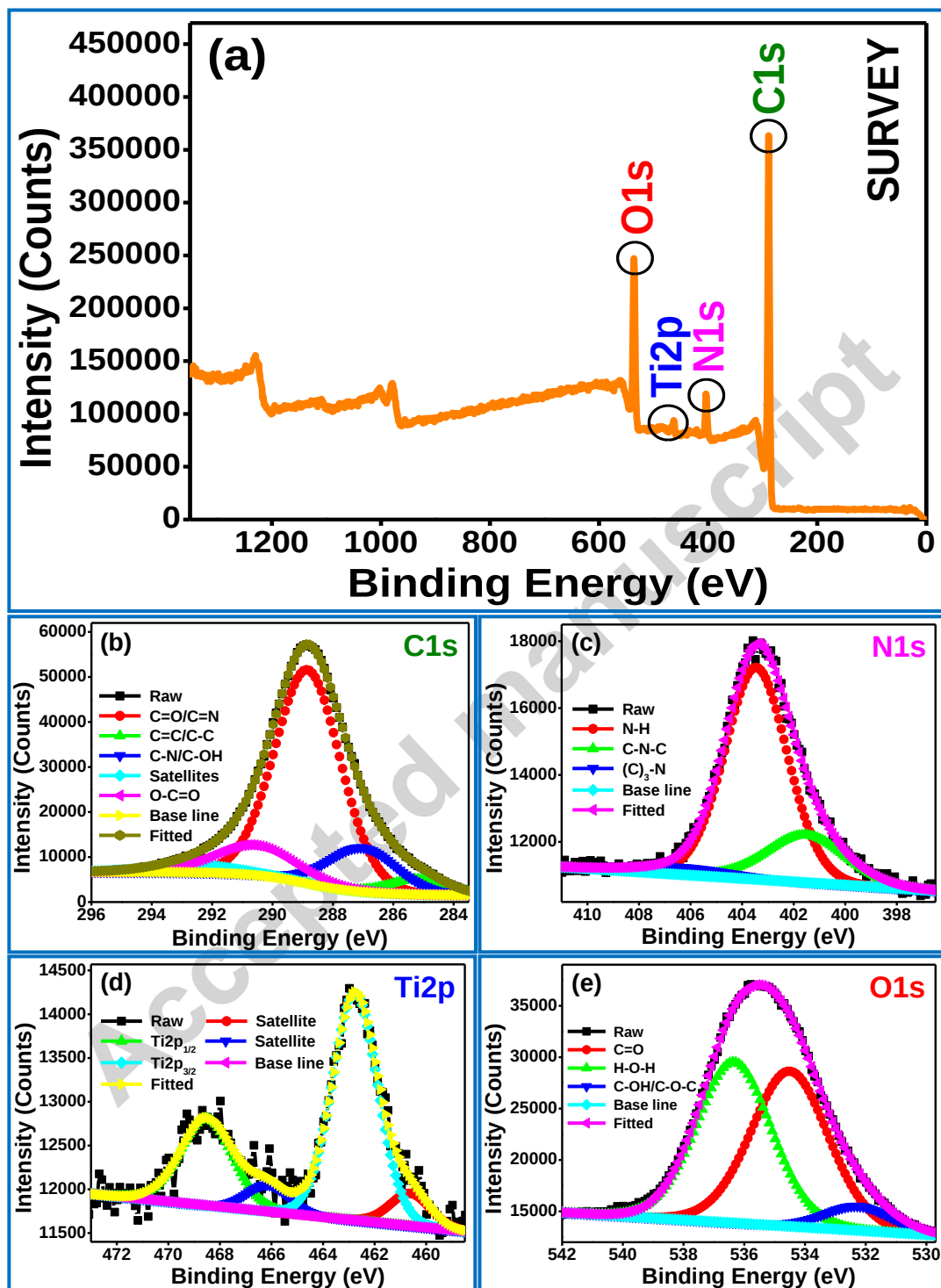
Fig. 2 (a) XPS survey scan spectrum and high-resolution spectra of (b) C 1s, (c) N 1s, (d) Ti
