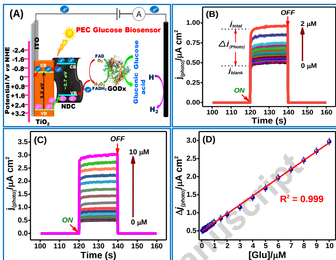
Fig. 4 (A) The schematic plausible mechanism for PEC Glu sensing at GODx/NDC-TiO 2 NPs/ITO. (B) The j_{(photo)}-t responses of GODx/NDC-TiO 2 NPs/ITO toward Glu at increasing concentration from 0 \mu M to 2 \mu M and (C) from 0 \mu M to 10 \mu M in the supporting electrolyte of 0.1 M pH 7.0. (D) Linear calibration ([Glu] vs. j_{(photo)} ) curve. Error bars indicate the standard deviation of three repeated measurements.
