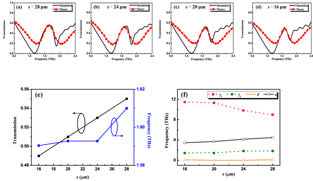
Fig.4 (a)-(d) The transmission curves obtained by simulation (black line) and theoretical calculations (red circles line) for s = 28, 24, 20 and 16 \mu\text{m} , respectively. (e) The dependence of transmission (black line) and resonant frequency (blue line) on the asymmetric degree s , respectively. (f) The dependence of \gamma_1 , \gamma_2 , \delta and \kappa extracted by fitting the transmission curves according to equation (2) on the asymmetric degree s , respectively. The unit of \kappa is \text{THz}^2 .
