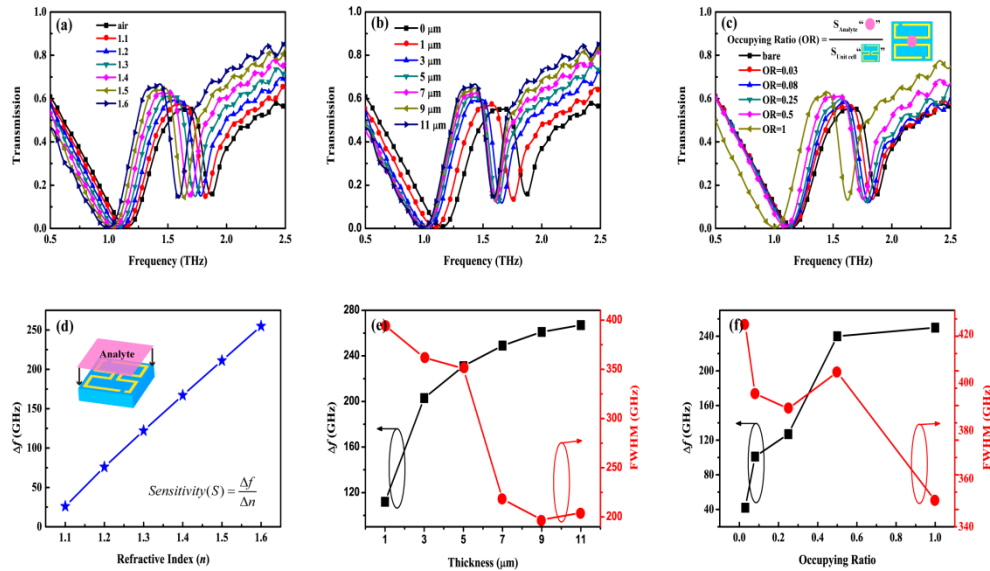
Fig.5 (a) The dependence of transmission on the analyte refractive index increasing from 1 to 1.6 under the thickness of 11 \mu\text{m} . (b) The dependence of transmission on the analyte thickness increasing from 0 to 11 \mu\text{m} under the fixed refractive index of 1.6. (c) The dependence of transmission on the occupying ratio (OR) increasing from 0.03 to 1 under the fixed refractive
