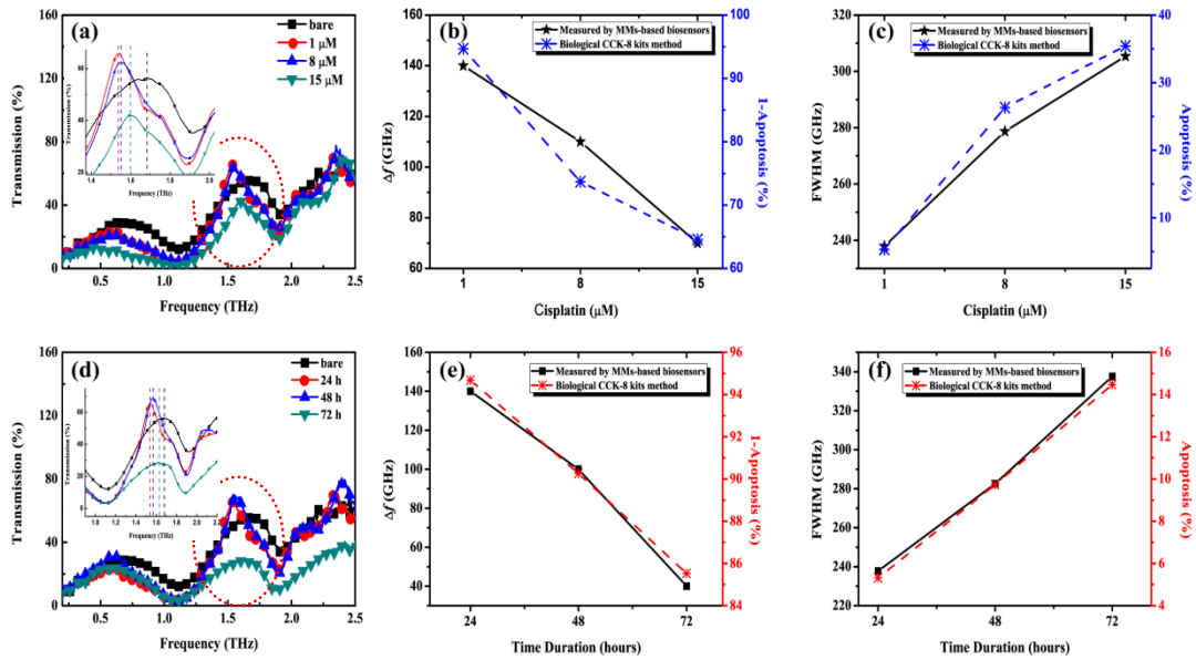
Fig.7 (a) The transmission of EIT-like MMs biosensors under different cisplatin concentrations from 1 to 15 \mu\text{M} , the bare case was also given for comparison. (b) The dependence of resonant peak shift \Delta f extracted from (a) and the apoptosis measured by the biological CCK-8 kits method
