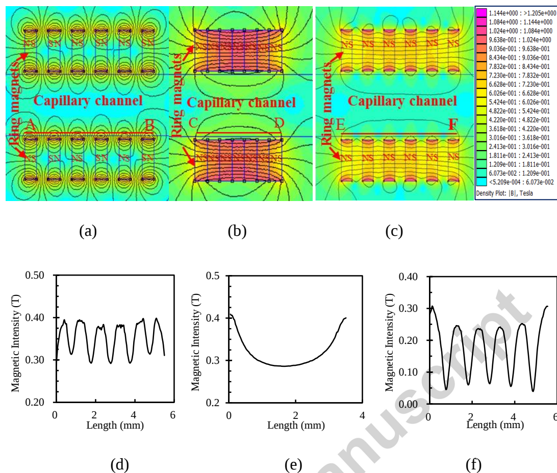
Fig. 1. (a)-(c) The simulation on the distribution of the magnetic field generated by the multi-ring magnets with three different layouts; (d)-(f) The distribution of the magnetic field in the capillary for three layouts.
