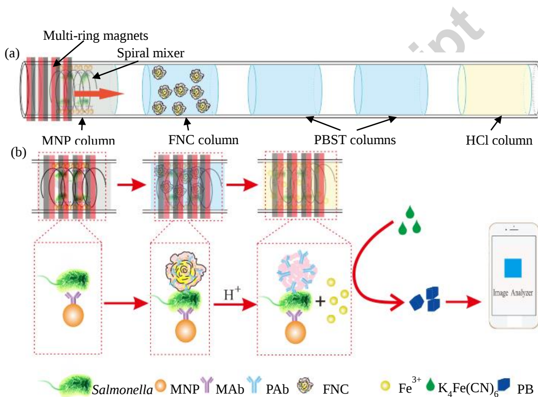
Scheme 1: (a) The capillary successively preloaded with the MNPs, the FNCs, PBST and HCl; (b)
