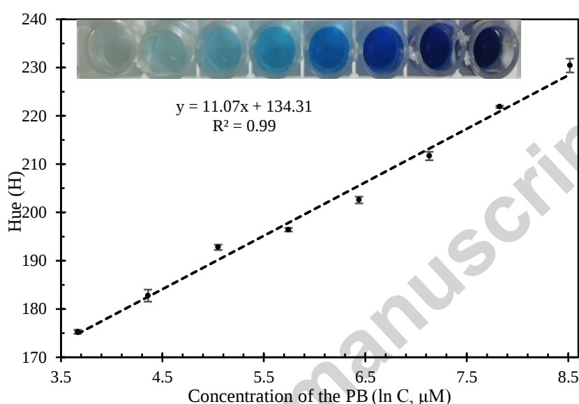
Fig. 2. The hue value for different concentrations of the PB from 39 \mu\text{M} to 5 mM
