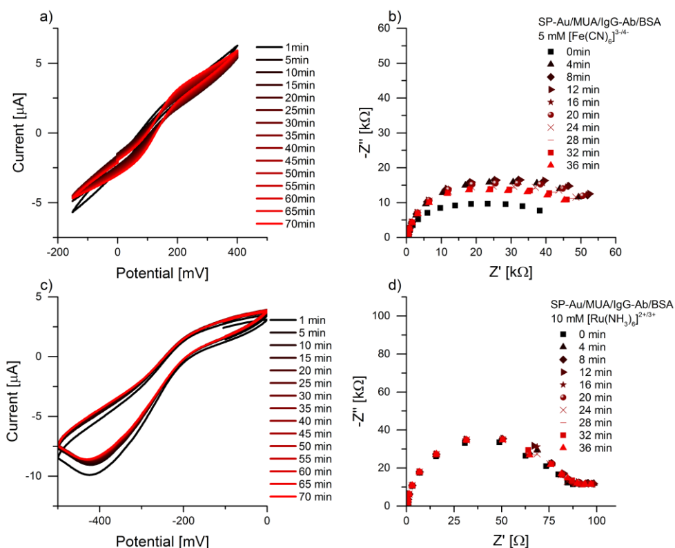
Fig. 4: a) CV over time of a MUA/IgG-Ab/BSA functionalized screen-printed sensor with 5 mM HCF as redox-probe; b) EIS spectra of a MUA/IgG-Ab/BSA functionalized screen-printed sensor with 5 mM HCF as redox-probe and a DC-bias 0.14 V; c) CV over time of a MUA/IgG-Ab/BSA functionalized screen-printed sensor with 10 mM Hexaammineruthenium (III) as redox-probe; d) EIS spectra of a MUA/IgG-Ab/BSA functionalized screen-printed sensor with 10 mM Hexaammineruthenium (III) as redox-probe and a DC-bias -0.16 V
