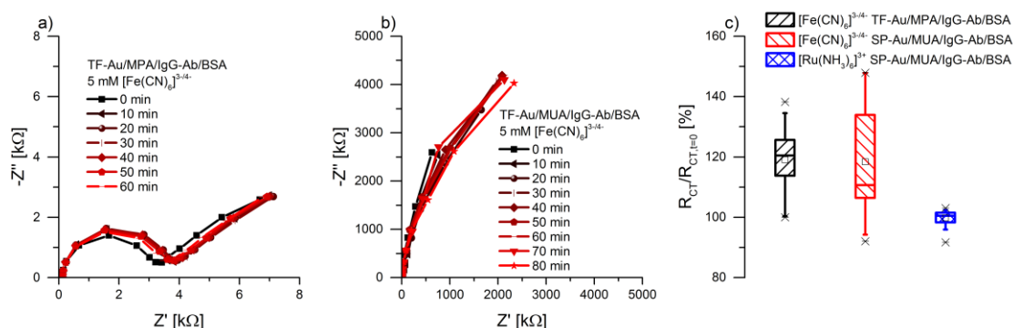
Fig. 2: a) EIS spectra over time of a MPA/IgG-Ab/BSA functionalized thin-film sensor with 5mM HCF as redox-probe; b) EIS spectra over time of a MUA/IgG-Ab/BSA functionalized thin-film sensor with 5mM HCF as redox-probe; c) Box plot for stability of biosensors over long measurement times of a MPA/IgG-Ab/BSA functionalized thin-film sensor (black) and a MUA/IgG-Ab/BSA functionalized screen-printed sensor (dark red) with 5 mM HCF in PBS as redox-probe, and a MUA/IgG-Ab/BSA functionalized screen-printed sensor with 10 mM [\text{Ru}(\text{NH}_3)_6]^{3+} in PBS as redox-probe (blue); each sensor was measured every two minutes over a period of 60 minutes, number of measurements m = 31 .
