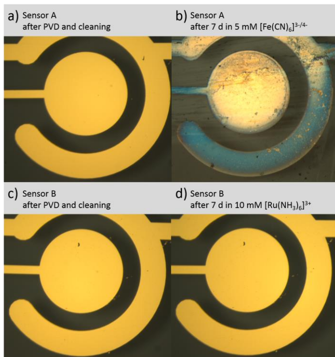
Fig. 3: a) Sensor A, new thin-film sensor after PVD and cleaning; b) Sensor A after 7 days of incubation in PBS with 5 mM HCF; c) Sensor B, new TF sensor after PVD and cleaning; d) Sensor B after 7 days of incubation in PBS with 10 mM Hexaammineruthenium (III).
