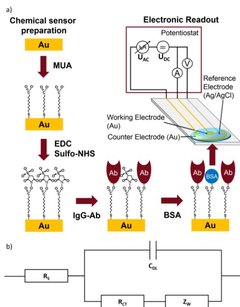
Fig. 1: a) Schematic of the sensor functionalization and the electronic readout; b) Randles circuit used for curve fitting
