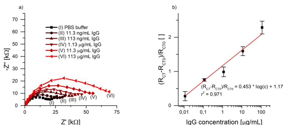
Fig. 5: a) Nyquist plots of a screen-printed biosensors with MUA/IgG-Ab/BSA functionalization after 30 minutes of incubation in (I) PBS, (II) 11.3 ng/mL IgG, (III) 113 ng/mL IgG, (IV) 1.13 \mu g/mL IgG, (V) 11.3 \mu g/mL IgG, and (VI) 113 \mu g/mL IgG; b) calibration curve of buffered IgG solutions with relative R_{CT} versus IgG concentration in half-logarithmic form, number of measurements m=3 .
