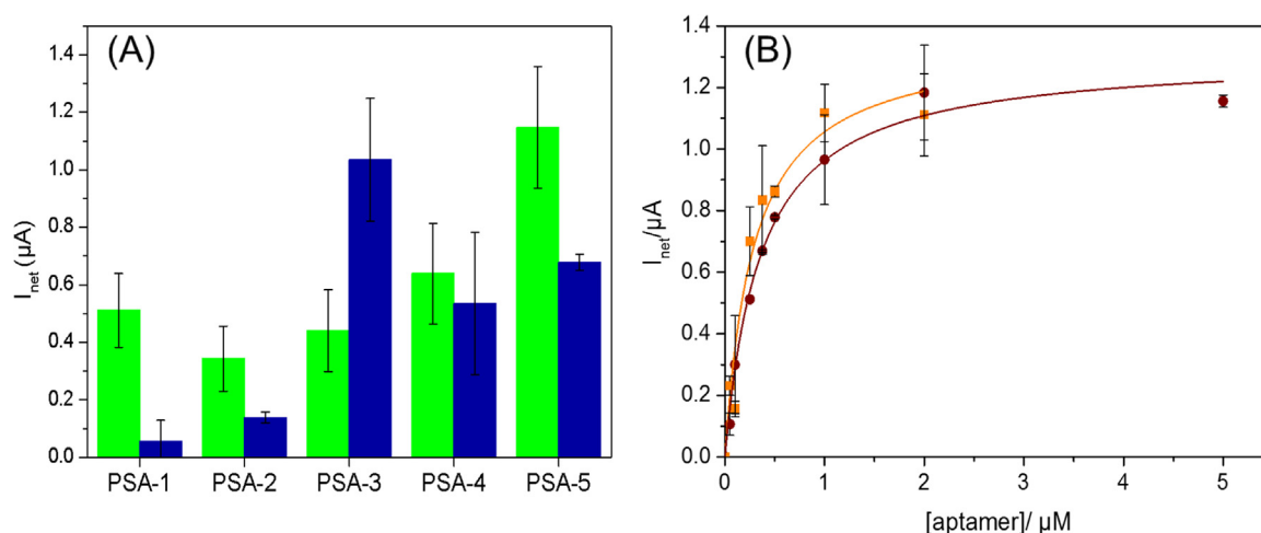
Fig. 3. A) Current intensities obtained by chronoamperometry at + 0.2 V on SPAuE modified with hPSA (light green) and rPSA (dark blue) using 500 nM of 6-FAM-aptamers. B) Binding curves obtained by chronoamperometry on hPSA-modified SPAuE for PSA-1 aptamer (circles) and anti-PSA (squares). (For interpretation of the references to color in this figure legend, the reader is referred to the web version of this article).
