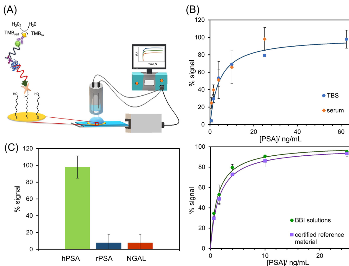
Fig. 4. A) Scheme of the sandwich assay, B) calibration plots of PSA in TBS, diluted serum 1:1 with TBS (upper panel) and two different PSA standards (bottom panel), and C) sensor response to 25 ng/mL of hPSA, rPSA and the glycoprotein NGAL.
