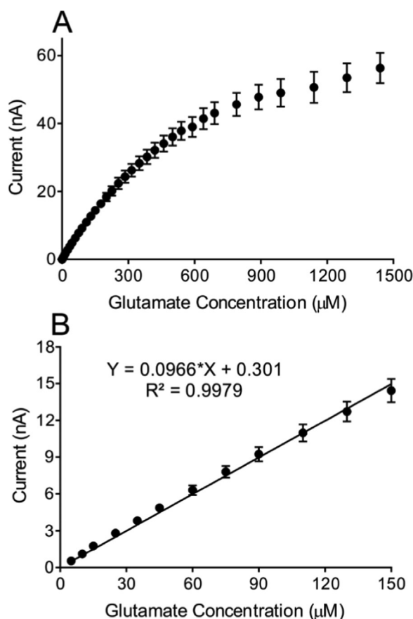
Fig. 3. (A) Glutamate biosensor calibration curve showing the sensor performance from 5 \mu\text{M} to 1500 \mu\text{M} glutamate. (B) Biosensor has a linear range up to 150 \mu\text{M} ( n = 21 ). Within the linear range the biosensor reliably measures glutamate with a sensitivity of 0.097 \text{nA}/\mu\text{M} .
