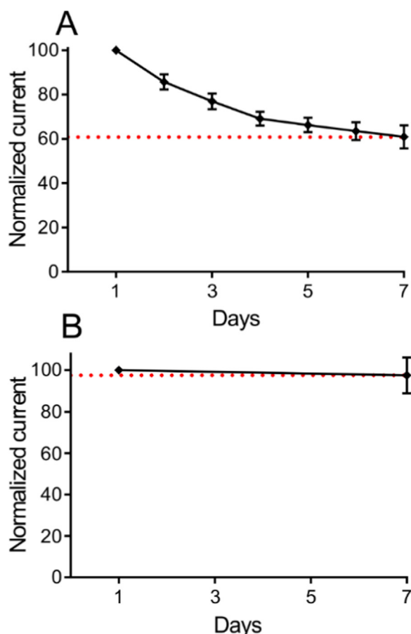
Fig. 5. Shelf life stability of glutamate biosensor. (A) The sensitivity of biosensors from Day 1 to Day 7 (Day 0 was the day of enzyme deposition). There was ~40% loss in average sensitivity ( n = 5 ) from Day 1 to Day 7. (B) Biosensors tested on Day1 and Day 7 shows ~5% loss in average sensitivity ( n = 7 ). In both studies, biosensors were stored under dry conditions at +4^{\circ}\text{C} between the tests.
