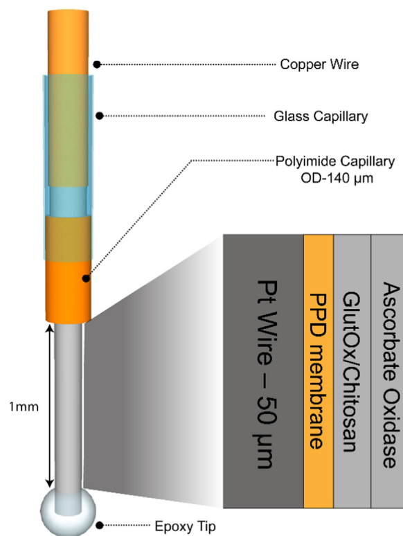
Fig. 1. Operational schematic of glutamate biosensor. The Pt wire is a 50 \mu\text{m} diameter and is coated with o-PD, GlutOx/Chitosan mixture, and AsOx. The wire has an epoxy tip at the protruding end to aid in enzyme deposition. The Pt wire is sheathed in a polyimide capillary (140 \mu\text{m} OD), which is subsequently inserted into a glass capillary tube. The top end of the Pt wire is connected to a copper wire via silver conducting epoxy; this copper wire makes contact with the potentiostat.
