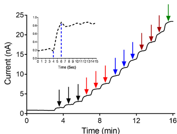
Fig. 2. Representative amperogram shows the biosensor response to glutamate. Applied potential is + 0.6 V vs Ag/AgCl. Arrows indicated with color coding are to indicate each of the individual concentrations tested in triplicate at 5 (black arrow), 10 (red arrow), 15 (blue arrow), and 20 \mu\text{M} (maroon arrow). Finally, one response to 25 \mu\text{M} (green arrow) is shown. Inset shows a response to 5 \mu\text{M} glutamate enlarged so that the time response can be seen. The sensor reaches its maximum in 2 s.
