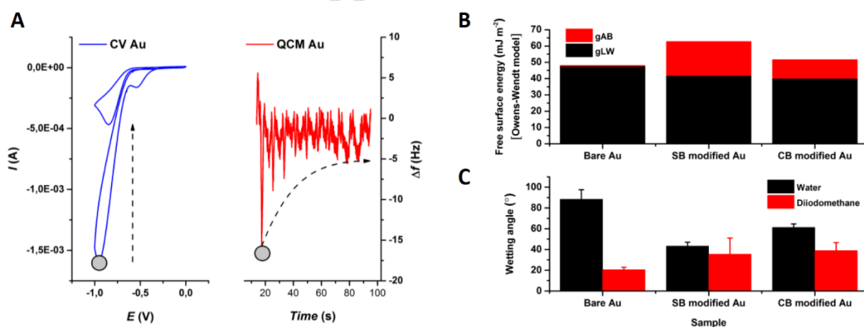
Fig. 2. EQCM of the preparation of zwitterionic SAM layer ( A ). A reduction peak occurs and decreases with each cycle at \sim -0.9\text{ V} vs. Ag/AgCl ( 1^{\text{st}} and 24^{\text{th}} scan, grey circle shows the 1^{\text{st}} scans reduction moment). Wetting angle (WA) measurement ( B,C ) using a two-liquid system with DW and diiodomethane. Free surface energy ( B ) was calculated using Owens-Wendt model. Bare Au electrode after polishing and gold oxide stripping procedure was strongly hydrophobic (WA \sim 88^\circ in DW). After the formation of CB/SB SAM layer, the interface becomes more hydrophilic with an increase in the polar component of the free surface energy due to the presence of zwitterions ( C ).
