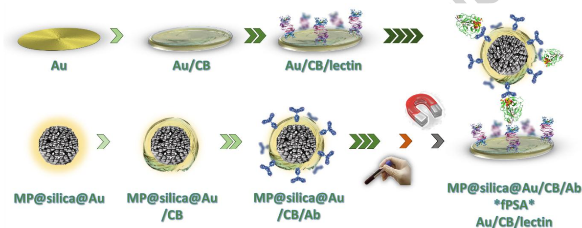
Scheme 1. Modification of Au electrode (upper row) using carboxybetaine aryldiazonium derivative (CB) and lectin (SNA-I). In the first step, carboxybetaine-bearing SAM layer was formed using cyclic voltammetry, and subsequently served for the covalent immobilization of a lectin. Lower row shows MP@silica@Au composite spontaneously modified with CB-derivative and subsequently with an antibody (Ab, anti-fPSA, chemically treated). After enrichment of fPSA from human sample using MP@silica@Au/CB/Ab by a permanent magnet, a sandwich was prepared and the signal was evaluated electrochemically.
