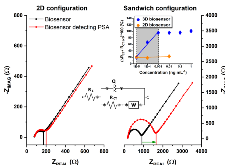
Fig. 3. The representative Nyquist plots for common 2D configuration (planar electrode interface modified using SAM layer and anti-fPSA antibody ( left ) and a sandwich-based configuration using MP@silica@Au clusters modified with anti-fPSA with an electrode modified using SNA-I lectin ( right ). EIS data were fitted using [R(Q[RW])] equivalent circuit (as showed in the inset ). A response towards 0.1 \text{ ng mL}^{-1} PSA in 10\times diluted real human serum is shown (red curves). A calibration curve for fPSA (blue) for a sandwich configuration is shown in the inset (error bars are too small to be visible). According to the slopes of calibration curves in the linear response range for both configurations, an amplification factor of 43 was calculated.
