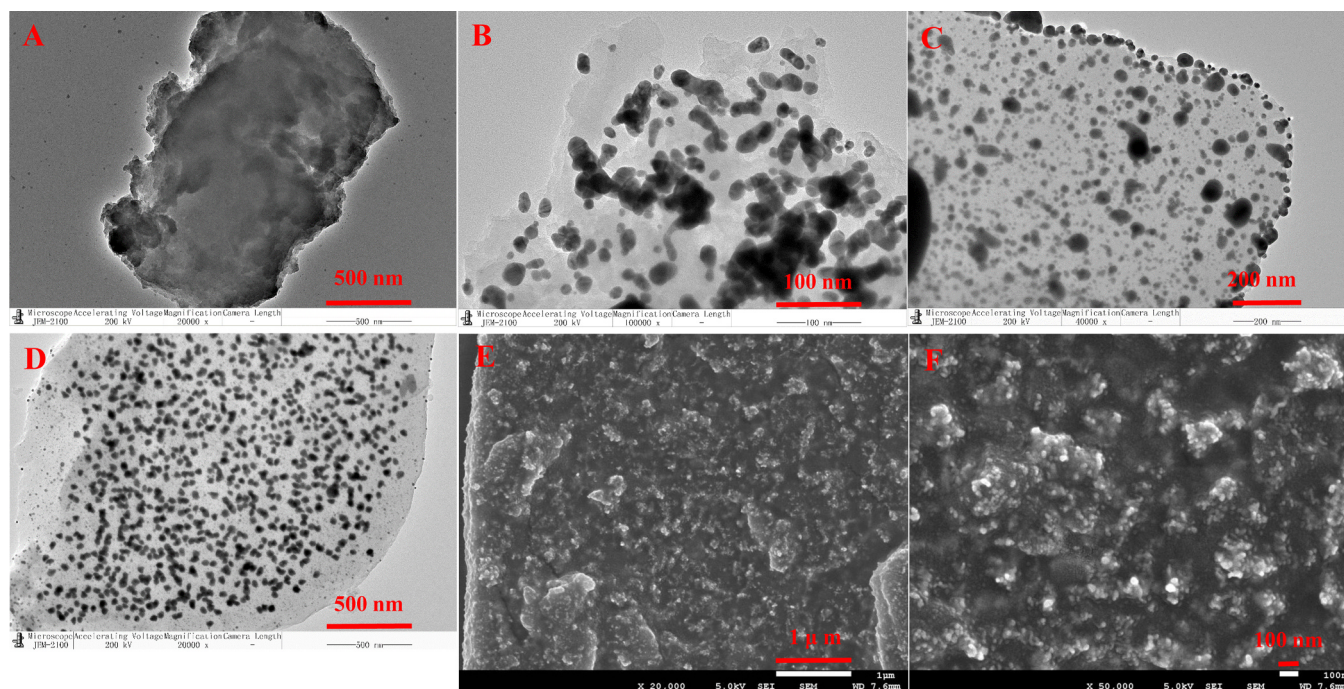
Fig. 1. TEM images of pristine GDY (A). TEM images of AuNPs-GDY compound with different masses ratio of GDY to tetrachloroauric acid: 1:3.75 (B); 1:2.5 (C); 1:1.875 (D). SEM images of AuNPs-GDY with the mass ratio of GDY to tetrachloroauric acid of 1:2.5 at different magnification (E, F).
