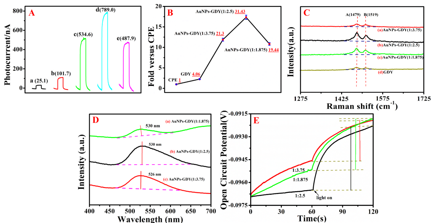
Fig. 2. (A) The PEC responses of bare CPE (a), GDY modified CPE (b), AuNPs-GDY modified CPE with mass ratio of GDY to tetrachloroauric acid of 1:3.75 (c), 1:2.5 (d), 1:1.875 (e). (B) The folds of PEC responses of different modified electrodes versus bare CPE. (C) The Raman spectroscopy of pristine GDY and AuNPs-GDY with different mass ratio of GDY to tetrachloroauric acid. (D) The ultraviolet spectroscopy of pristine GDY and AuNPs-GDY with different mass ratio of GDY to tetrachloroauric acid. (E) The open circuit potential AuNPs-GDY. The PEC and OCPT were carried out in pH 7.4 PBS contained 10 \mu\text{M} AA.
