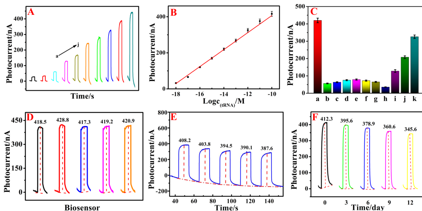
Fig. 4. (A) PEC responses of the PEC biosensor toward different concentrations of let-7a. From a to j: 0, 0.001, 0.01, 0.1, 1, 10, 100, 1000, 10000, 100000 fM. (B) The linear relationship of the PEC responses to the logarithm of let-7a concentration. (C) Selectivity and specificity of the designed PEC biosensor. a to h: let-7a, let-7b, let-7c, let-7d, let-7e, let-7f, let-7g (The concentrations of let-7a and six other let-7 microRNA family were 100 pM and 10 nM, respectively); h: blank; i: 100 fM let-7a; j: serum sample; k: mixture of 100 fM let-7a and human serum, respectively. (D) Reproducibility of designed PEC biosensor. Five biosensors were tested in parallel. (E) Time-based photocurrent responses of the PEC biosensor. (F) Stability of designed PEC biosensor for 12 days storage: 0st, 3rd, 6th, 9th, 12th. The concentration of let-7a was 100 pM in 0.1 M pH 8.0 PBS contained 10 mM AAP.
