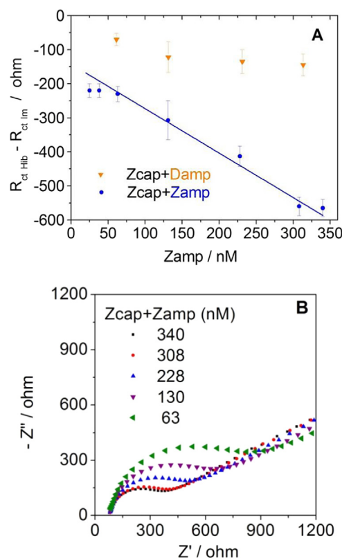
Fig. 4. (A) Analytical curve of charge transfer resistance ( \Delta R_{ct} = R_{ct} \text{ Hib} - R_{ct} \text{ Im} ): (A) Immobilization of 0.40 \mu M of the capture sequence (Zcap) for 5 h at 45 °C. Hybridization with Zamp, blue circle (●) at concentrations of 25, 38, 63, 130, 228, 308 and 340 nM and negative control with Damp, orange triangle (▼) at the concentration of 63, 130, 228 and 308 nM. (B) Nyquist plots after Zcap + Zamp hybridization at five concentrations included in the linear region. EIS performed in a drop of 60 \mu L , three separate electrodes for each concentration ( n = 3 ).
