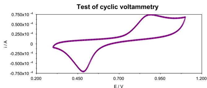
Fig. 2. Cyclic voltammogram for SOxNPs/AuE in 25 ml 0.1 M sodium phosphate buffer (pH = 6.5) containing 2 mM (0.1 ml) sarcosine at a scan rate of 20 mVs -1 .
