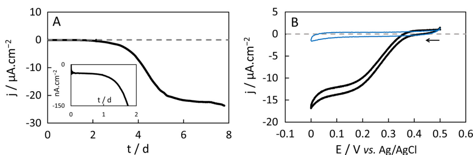
Fig. 2. (A) Increase of cathodic current associated with EAB growth in unamended tap water, glassy carbon RDE polarized at +0.2 \text{ V vs. Ag/AgCl} , 160 rpm, under air, inoculation at t = 0 . The inset displays a zoom on the two first days. (B) Representative cyclic voltammograms of a mature EAB in tap water under air (thick black line) or anoxic conditions (thin blue line), at 0.2 \text{ mV s}^{-1} .
