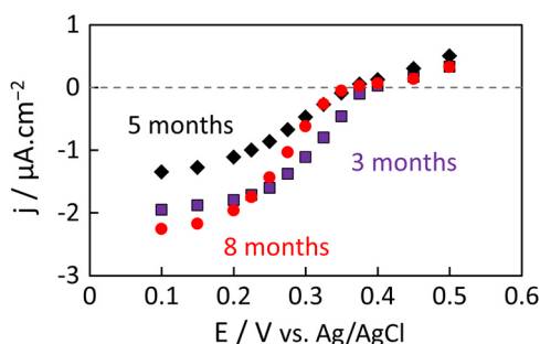
Fig. 5. Polarization curves of a cathodic EAB on graphite rod after 3 months (purple squares), 5 months (black lozenges) and 8 months (red circles) of continuous polarization at +0.1 V vs. Ag/AgCl in tap water refreshed every few days in a recirculating setup as schematized in Fig. 1. The polarization curves were obtained by successive chronoamperometries recorded at decreasing potentials and the current reported are at quasi steady-state.
