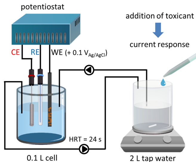
Fig. 1. Principle of the recirculating setup for assessing EABs responses to toxic shocks. CE, RE and WE stands for counter, reference and working electrode, respectively.
