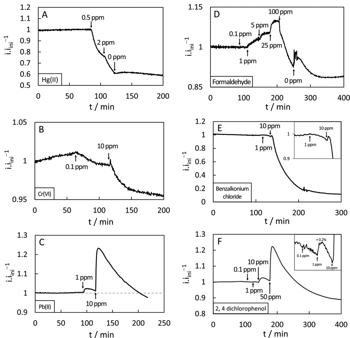
Fig. 4. Toxic shocks monitored for several heavy metals: (A) Hg(II), (B) Cr(VI), (C) Pb(II); and organic toxicants: (D) formaldehyde, (E) benzalkonium chloride, (F) 2, 4 dichlorophenol. Currents are normalized with respect to the initial baseline current in absence of toxicant. The additions of toxic compounds are represented by arrows with the corresponding new concentrations of the toxic element; '0 ppm' correspond to a replacement of the contaminated water by fresh tap water devoid of contaminant. Zooms in inset for smaller impacts. Baseline currents are provided in Table S3. Note differences in scales.
