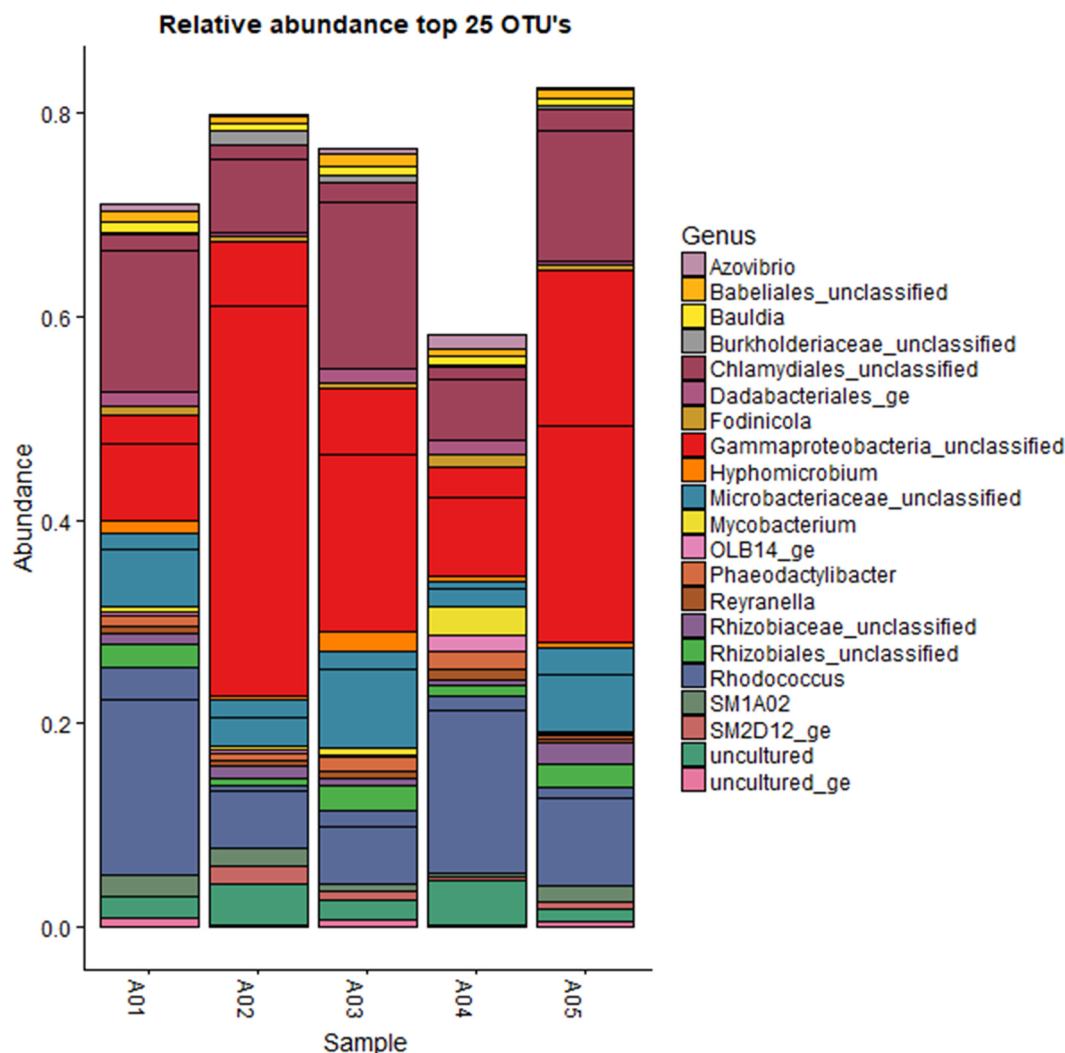
Fig. 3. Relative abundance of the microbial communities harvested on five O_2 -reducing EABs. Only the top 25 OTUs are represented.
