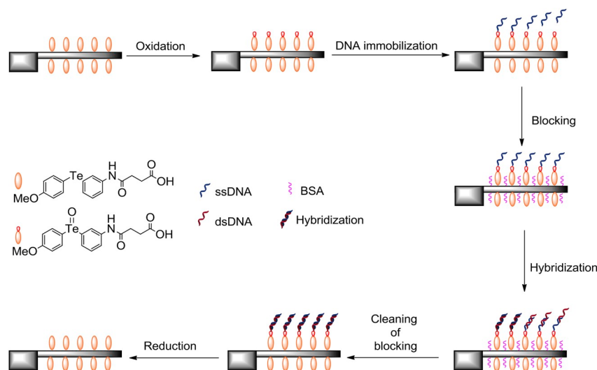
Scheme 1. Schematic representation of the immobilization process using telluride and DNA sequences. In this system, telluroxide was formed only on the active surface of the microcantilever to ensure the detection response.
