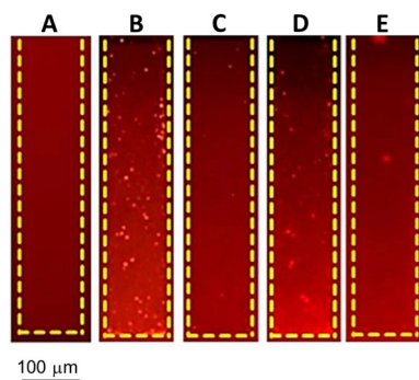
Fig. 4. Images obtained during two DNA immobilization processes: (A) Telluride compound immobilization, (B) first immobilization of T5 DNA-SH-CY3, (C) first reduction of telluride, (D) second immobilization of T5 DNA-SH-CY3 and (E) second reduction of telluride.
