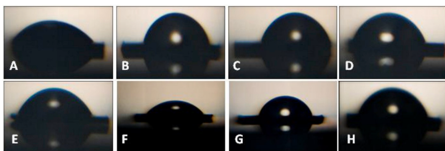
Fig. 1. Surface analysis: A-oxidation with piranha solution, B- APTES self-assembled monolayer, C- telluride (3a) immobilization, D-oxidation of telluride, E- DNA immobilization, F- surface blocking (BSA), G-complementary strand (ds-DNA) and H- reduction of telluride (surface regeneration). The graph illustrates the layer thickness variation of each process by ellipsometry: SiO 2 ( 1.960 \pm 0.08485 nm), APTES ( 1.554 \pm 0.1389 nm), Te ( 0.7980 \pm 0.2376 nm), DNA-SH ( 0.3040 \pm 0.1624 nm) and DTT ( 0.8420 \pm 0.06686 nm) (one-way ANOVA: Tukey Test).
